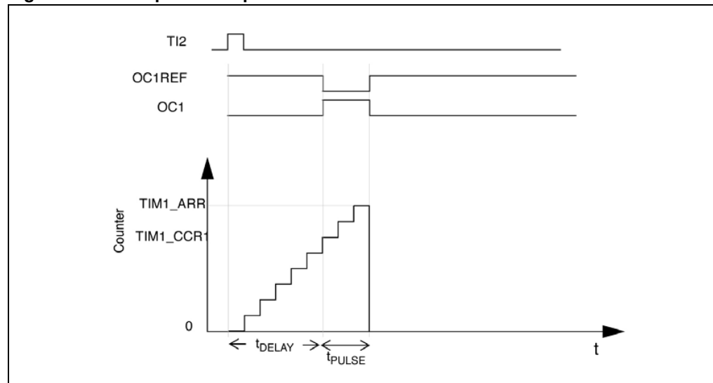
Figure 37. Example of one pulse mode
