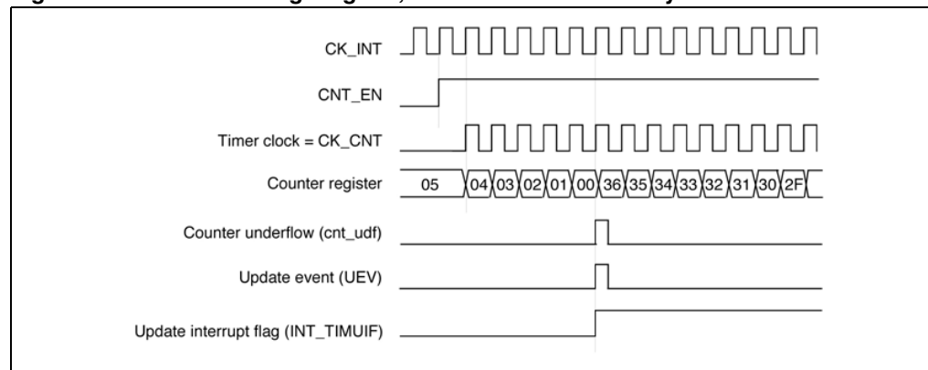
Figure 20. Counter timing diagram, internal clock divided by 1
