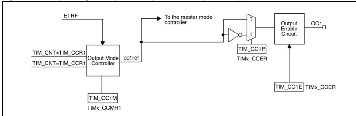
Figure 32. Output stage of capture/compare channel (channel 1)
