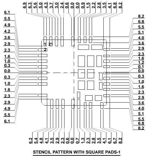
STENCIL PATTERN WITH SQUARE PADS-1
