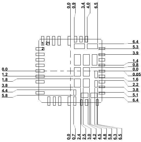
STENCIL PATTERN WITH SQUARE PADS-2
