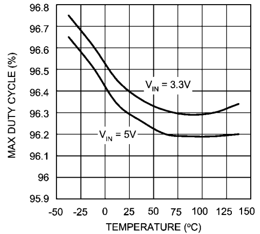
Max. Duty Cycle vs Temperature - "Y"
