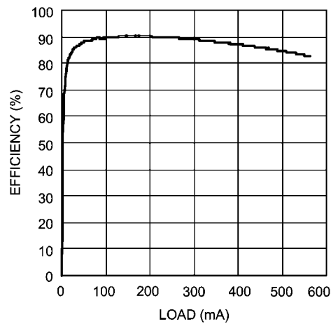
Efficiency vs Load Current - "Y" V_{IN} = 5V, V_{OUT} = 12V
