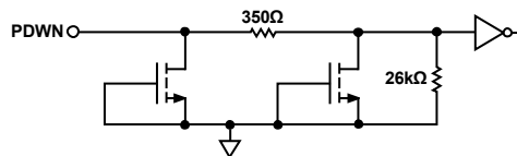
Figure 76. Equivalent PDWN Input Circuit
