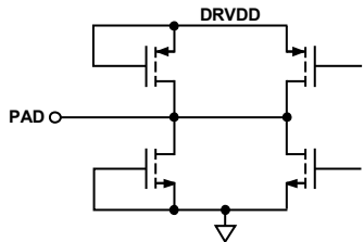
Figure 70. Digital Output
