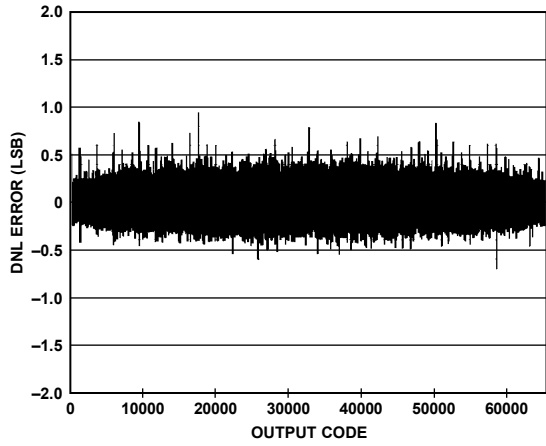
Figure 47. AD9650-80 DNL with f_{IN} = 9.7 MHz
