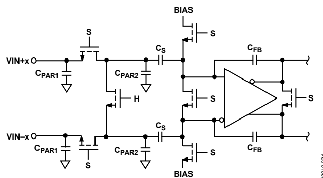
Figure 77. Switched-Capacitor Input
