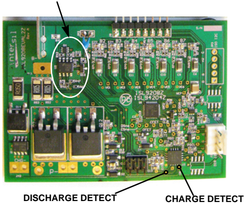
FIGURE 8. ISL9208EVAL2Z CURRENT DETECTION CONNECTIONS
