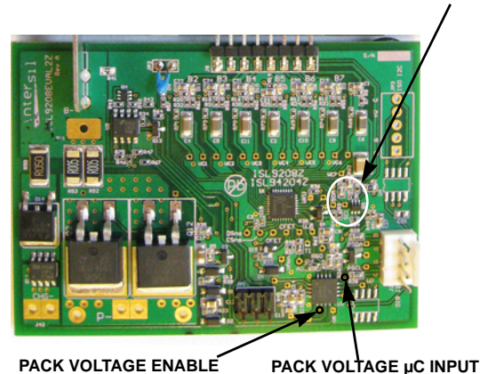
FIGURE 10. ISL9208EVAL2Z PACK VOLTAGE MONITORING CONNECTIONS
