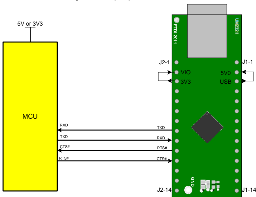
Figure 7.1 : Bus Powered Configuration
