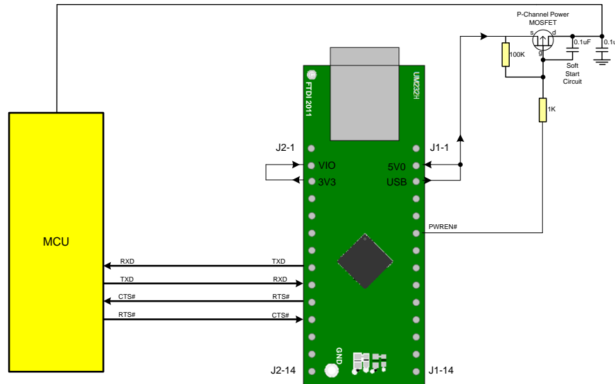
Figure 7.2 : Bus Powered with Power Switching Configuration
