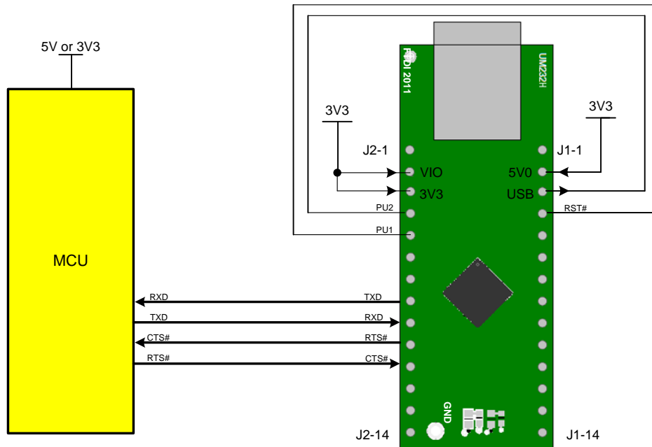
Figure 7.5 : Self-Powered Configuration – 3V3 External Supply
