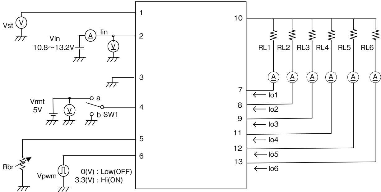
RL1 to 6: Load resistance (600Ω, 20W min.)
