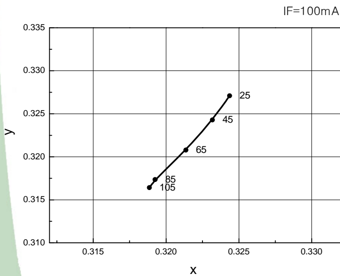
Junction Temperature ( ^{\circ}\text{C} ) vs. Chromaticity Coordinate
