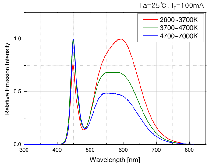
Spectrum
