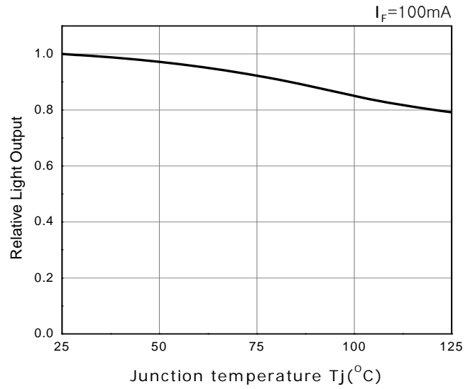
Relative Light Output vs. Junction Temperature
