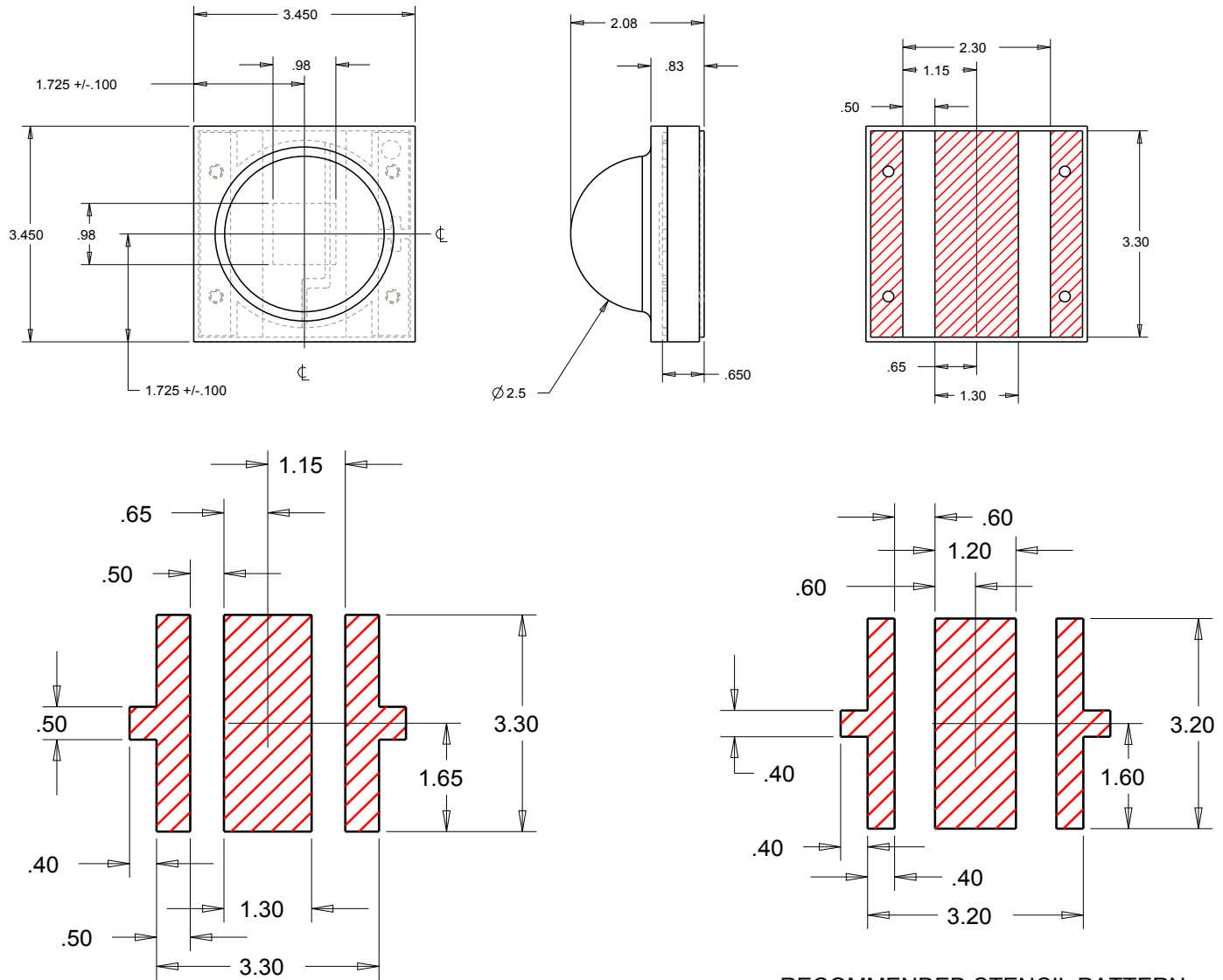
RECOMMENDED STENCIL PATTERN (HATCHED AREA IS OPENING)
