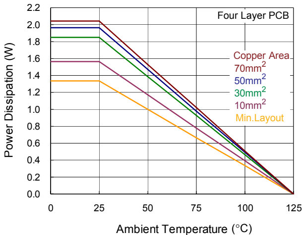
Figure 5. Derating Curves for RT8289 Package
