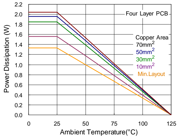
Figure 7. Derating Curves for RT8293A Package
