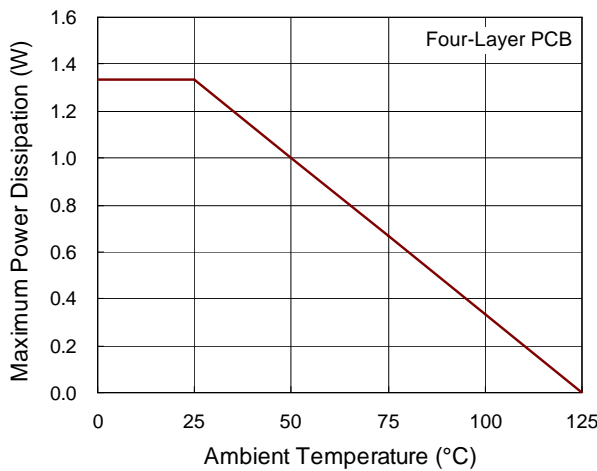
Figure 3. Derating Curve for RT8290 Package
