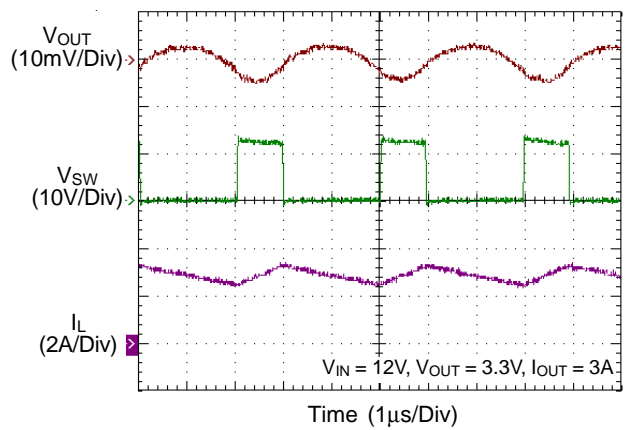
Switching Waveform
