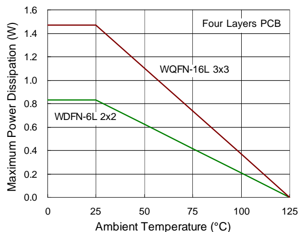
Figure 5. Derating Curves for RT8010/A Package
