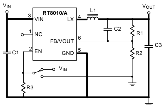
Figure 6. EVB Schematic
