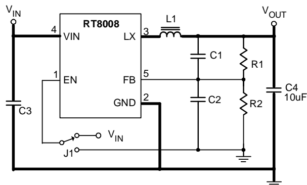
Figure 6. EVB Schematic
