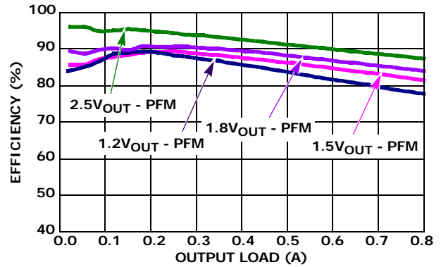
FIGURE 2. EFFICIENCY vs LOAD 2.25MHz 3.3VIN PFM
