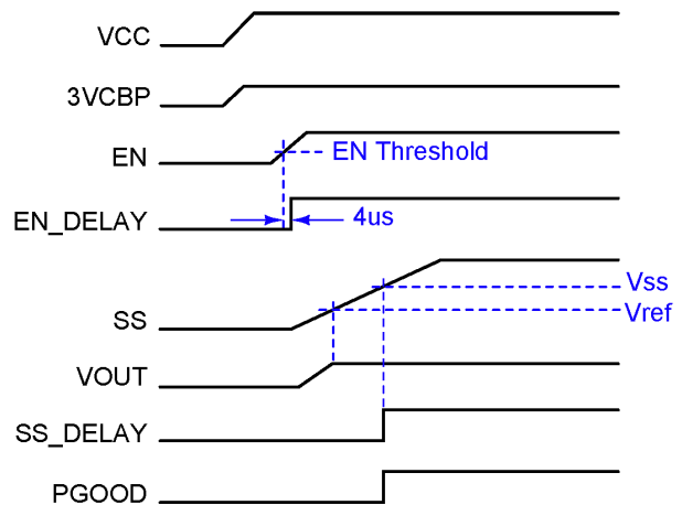
Figure 20. Normal Startup
