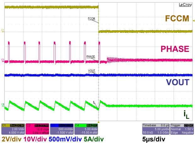
Figure 17: FCCM/DCM Transition
