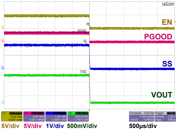
Figure 9: Shutdown
