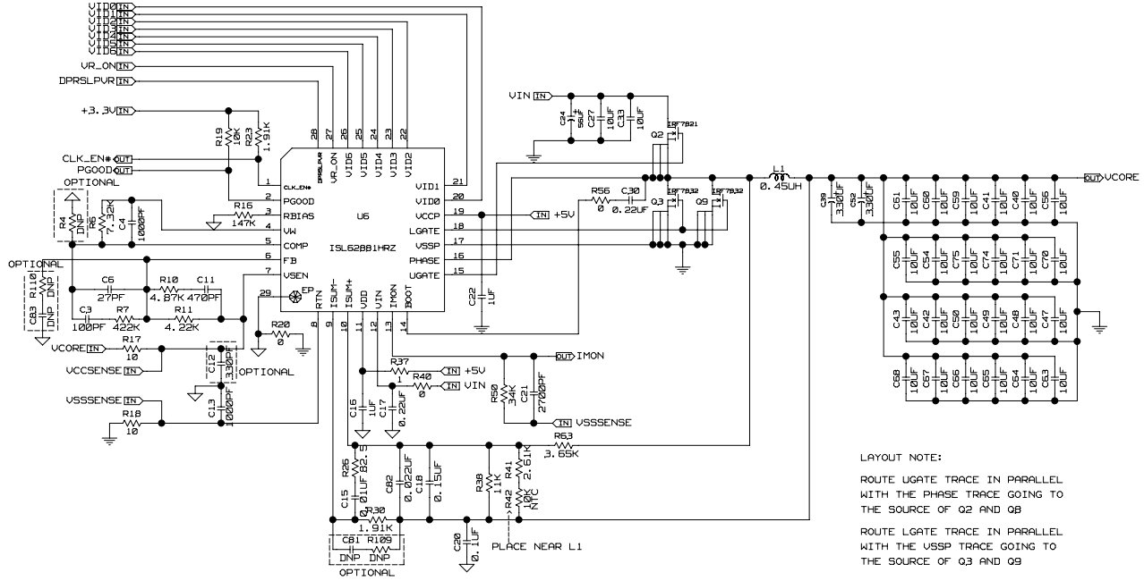
FIGURE 26. CPU APPLICATION REFERENCE DESIGN
