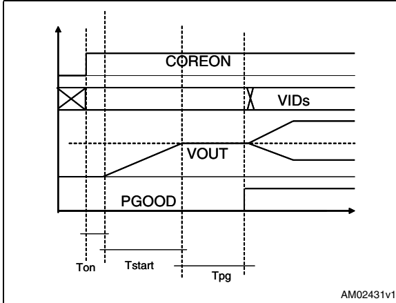
Figure 34. IMVP6.5 GFX mode start-up
