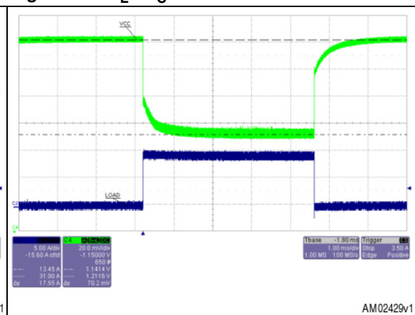
Figure 32. \tau_L < \tau_C
