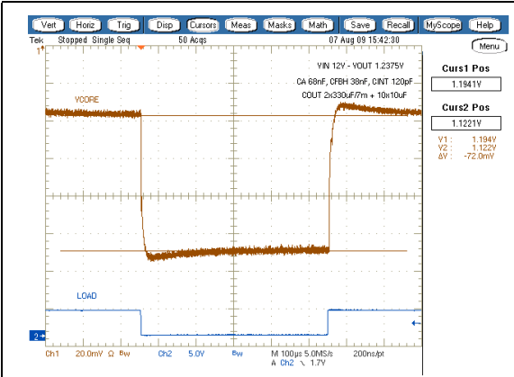
Figure 47. C15 good and C34 big
