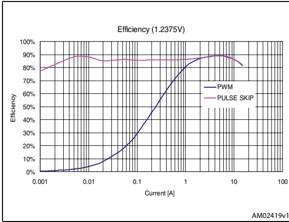
Figure 22. V_{CORE} efficiency (DPRSLPVR high and low)
