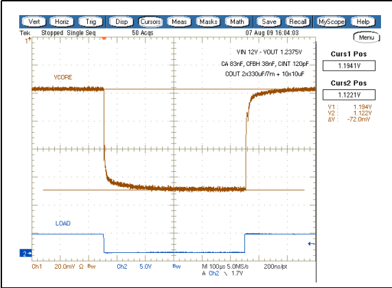
Figure 45. C15 small and C34 OK
