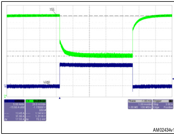
Figure 37. Average current limit - recovery
