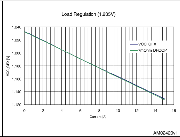
Figure 23. V_{CORE} load regulation - droop function
