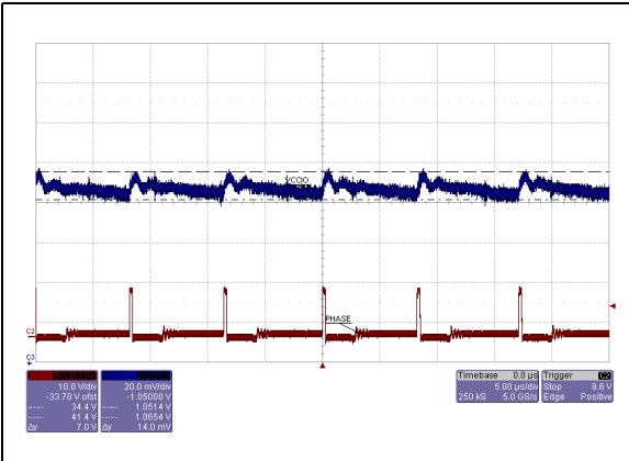
Figure 51. VCCIO output voltage ripple (1 A)
