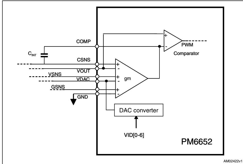
Figure 25. PM6652 integrator
