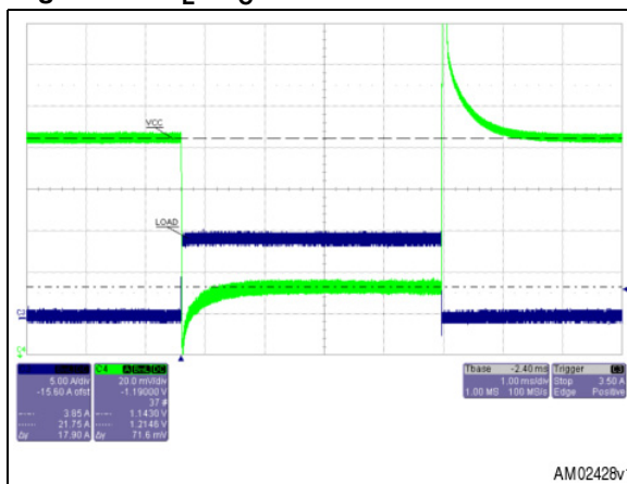
Figure 31. \tau_L > \tau_C
