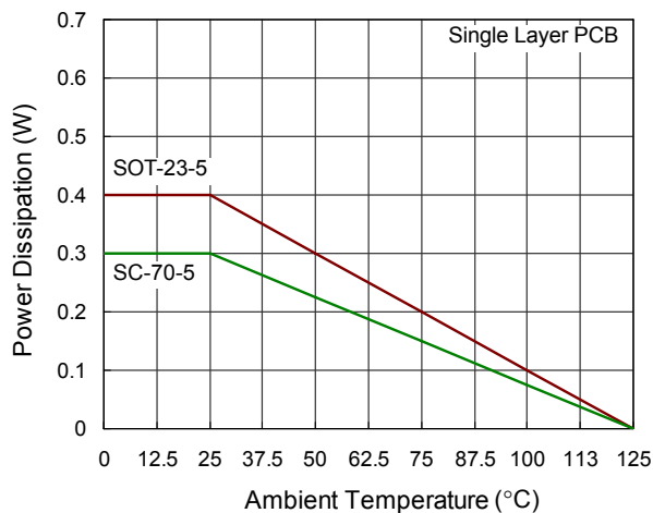
Figure 2. Derating Curves for RT9020 Packages
