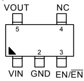
TSOT-23-5/SOT-23-5/ SC-70-5 (R-Type)
