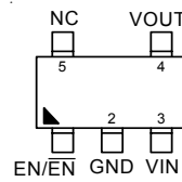
TSOT-23-5/ SOT-23-5(G-Type)
