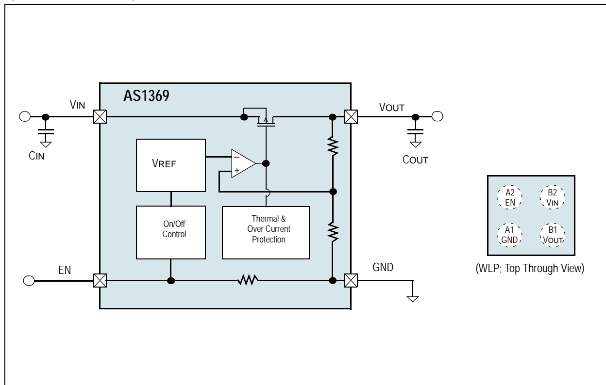
Figure 1. AS1369 - Block Diagram
