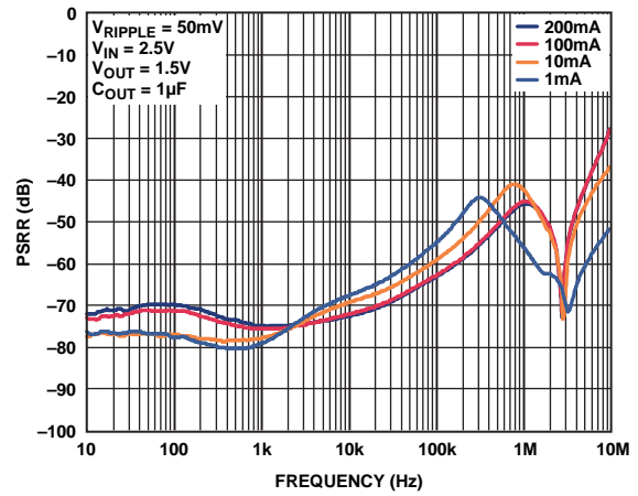
Figure 32. Power Supply Rejection Ratio vs. Frequency, 1.5 V
