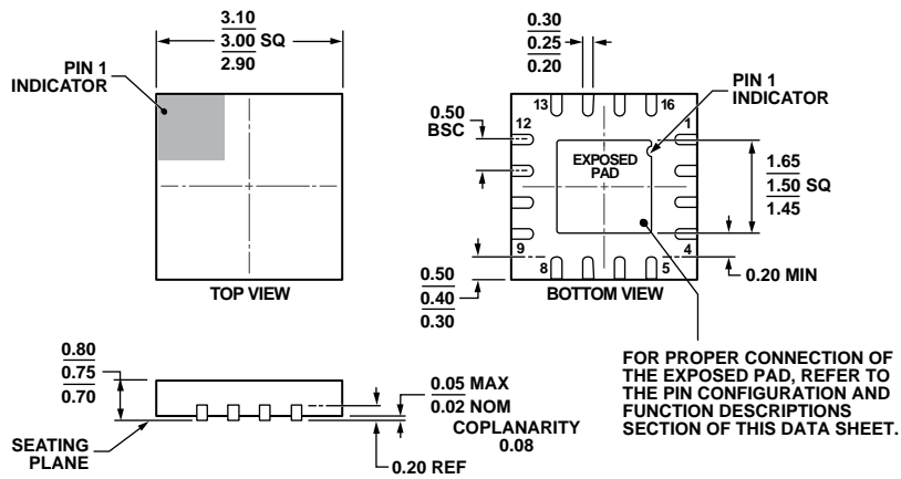
Figure 56. 16-Lead Lead Frame Chip Scale Package [LFCSWQ] 3 mm × 3 mm Body, Very, Very Thin Quad (CP-16-27) Dimensions shown in millimeters
