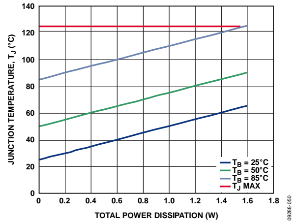
Figure 53. Junction Temperature vs. Total Power Dissipation and Board Temperature
