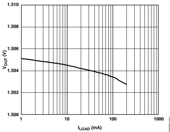
Figure 12. Output Voltage vs. Load Current
