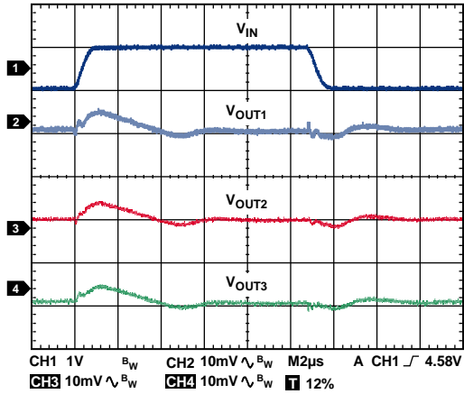
Figure 41. Line Transient Response, V_{IN} = 4\text{ V to }5\text{ V} , I_{LOAD1} = I_{LOAD2} = I_{LOAD3} = 1\text{ mA} , CH1 = V_{IN} , CH2 = V_{OUT1} , CH3 = V_{OUT2} , CH4 = V_{OUT3}
