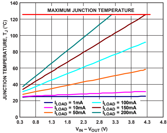
Figure 42. 100 mm 2 of PCB Copper, WLCSP, T A = 50°C
