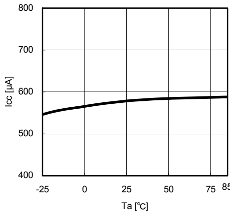
Fig.8 Ta-Icc
