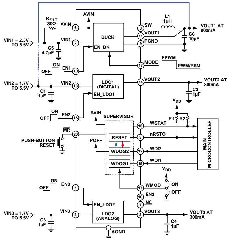
Figure 69. Application Diagram
