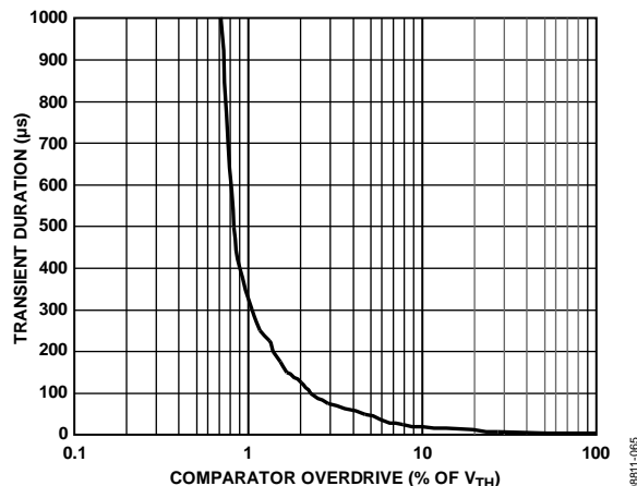
Figure 64. Maximum V_{TH} Transient Duration vs. Reset Threshold Overdrive
