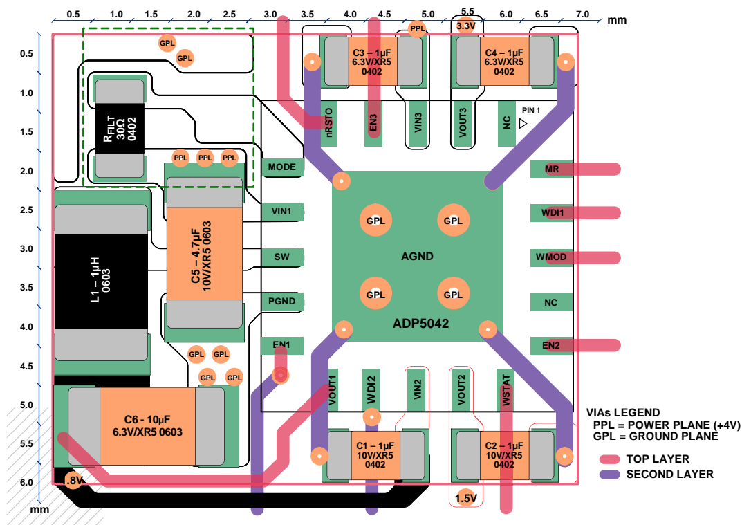
Figure 68. Layout
