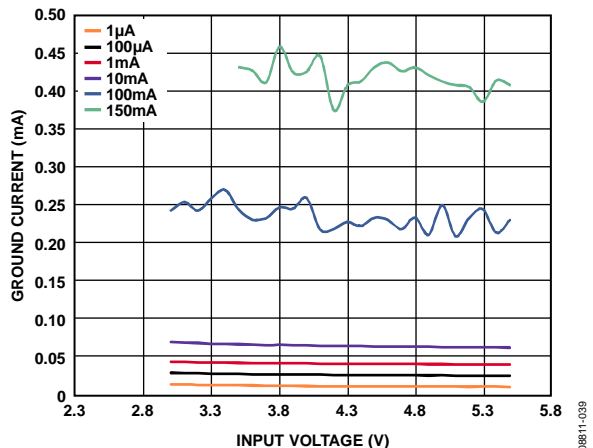
Figure 39. LDO2 Ground Current vs. Input Voltage, Across Output Load, VOUT3 = 2.8 V
