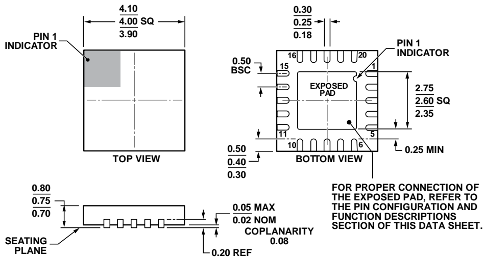
Figure 70. 20-Lead Lead Frame Chip Scale Package [LFCSP_WQ] 4 mm × 4 mm Body, Very Very Thin Quad (CP-20-8)
