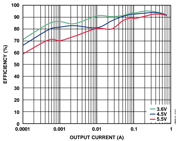
Figure 11. Buck Efficiency vs. Load Current, Across Input Voltage, V_{OUT1} = 3.3\text{ V} , Auto Mode
