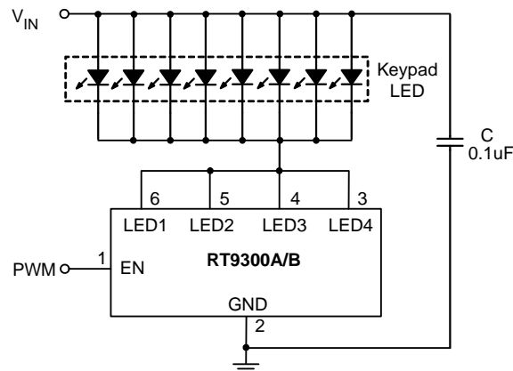
Figure 2. Application Circuit for Keypad.
