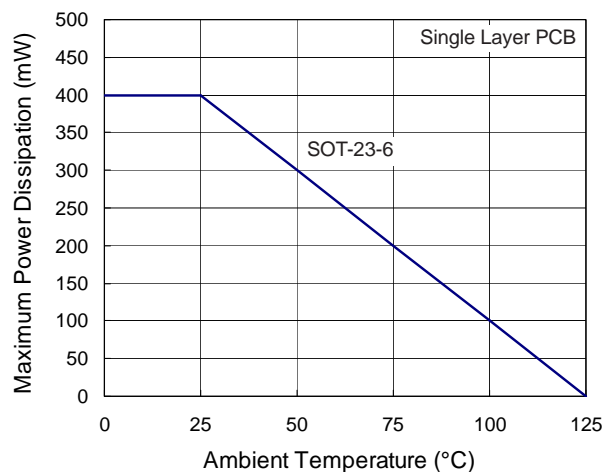
Figure 1. Derating Curves for RT9300 Packages
