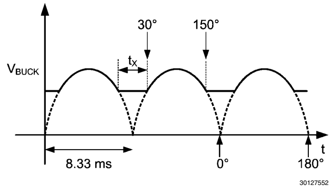
FIGURE 11. Two Stage Valley-Fill V_{BUCK} Voltage
