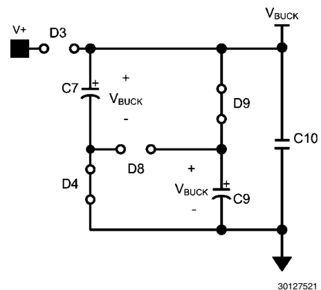
FIGURE 5. Two stage Valley-Fill Circuit when AC Line is Low
