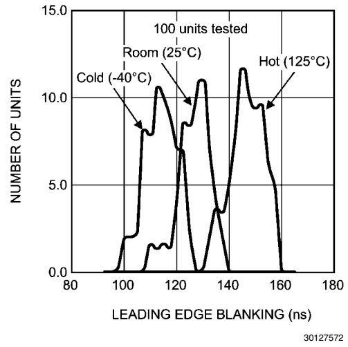
Leading Edge Blanking Variation Over Temperature
