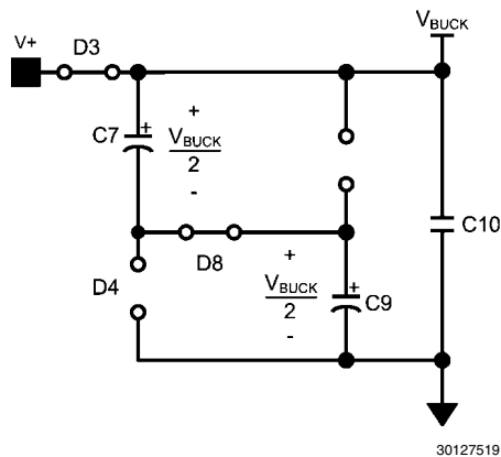
FIGURE 4. Two stage Valley-Fill Circuit when AC Line is High
