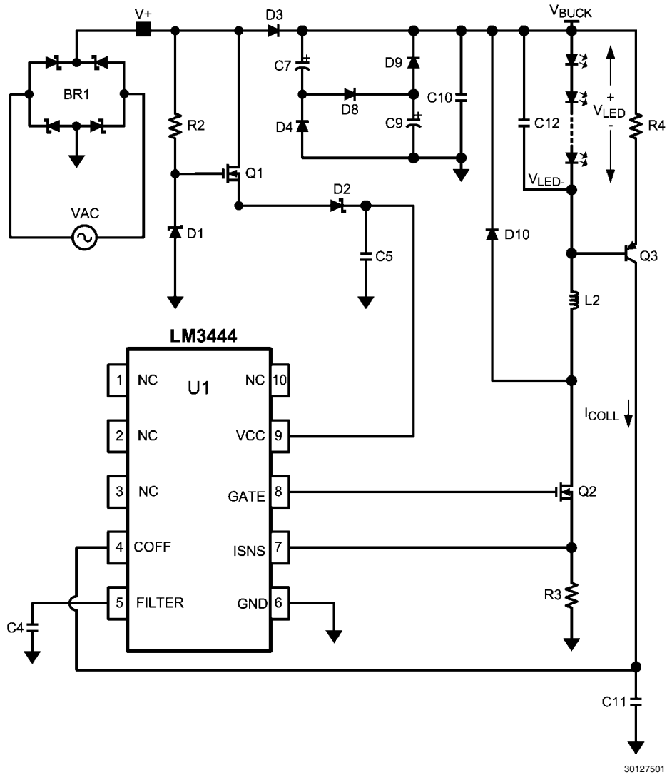
FIGURE 2. LM3444 Schematic
