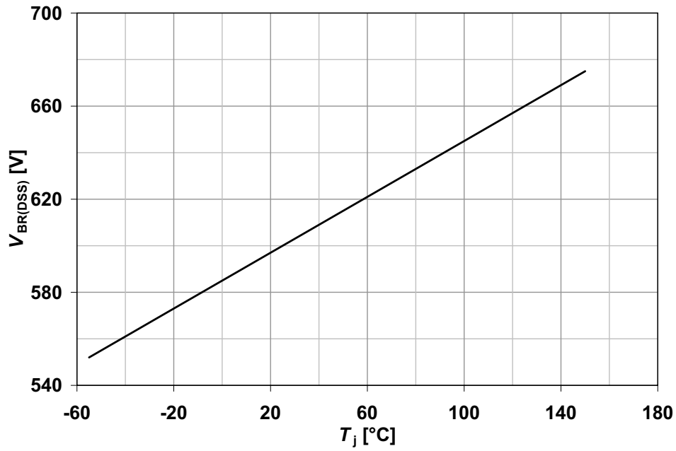
Figure 11 Drain-source breakdown voltage; V_{BR(DSS)}=f(T_j)
