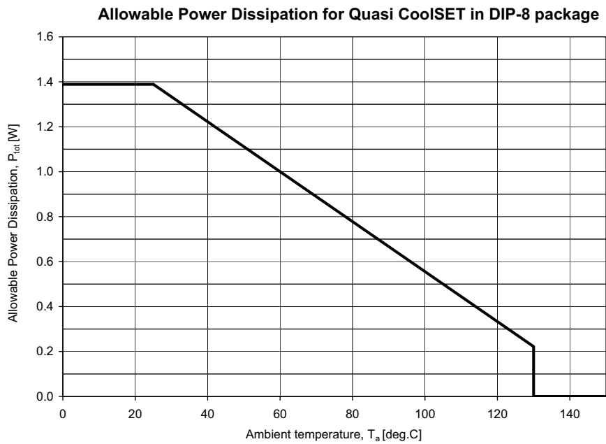
Figure 10 Power dissipation; P_{tot}=f(T_a)
