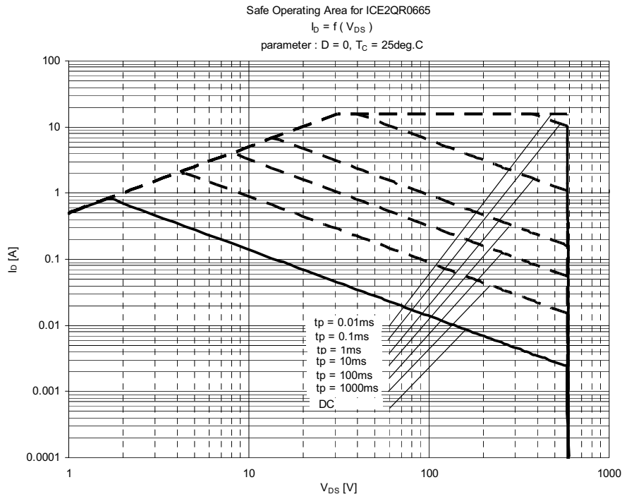
Figure 9 Safe Operating Area(SOA) curve for ICE2QR0665
