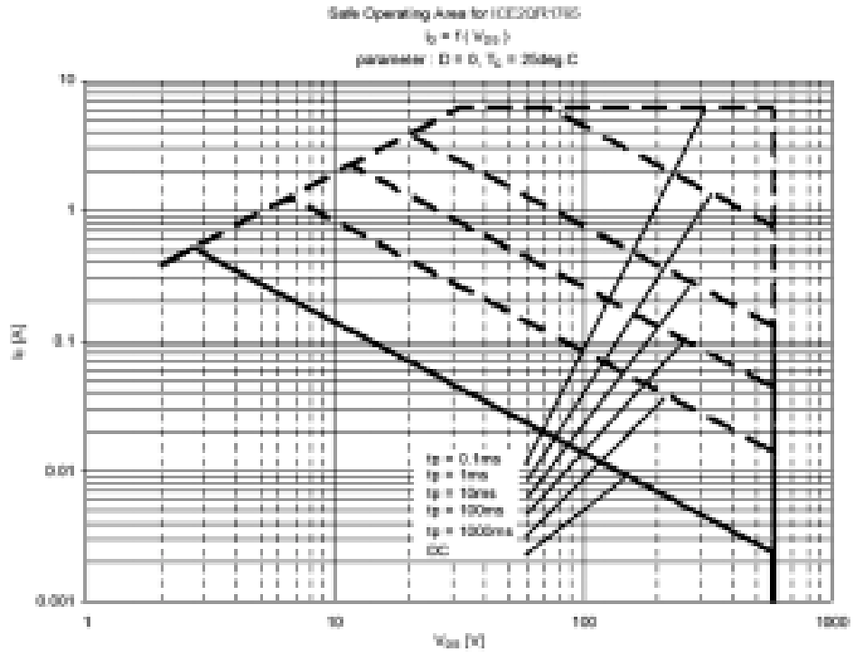
Figure 9 Safe Operating Area(SOA) curve for ICE2QR1765
