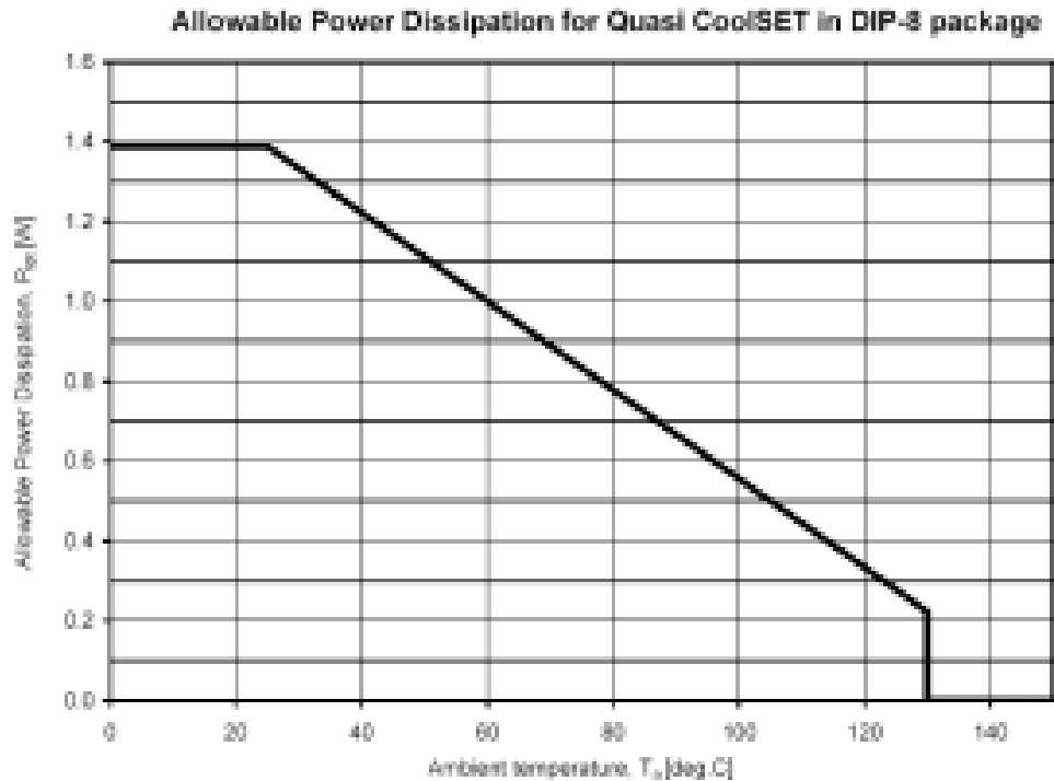
Figure 10 Power dissipation; P_{tot} = f(T_a)
