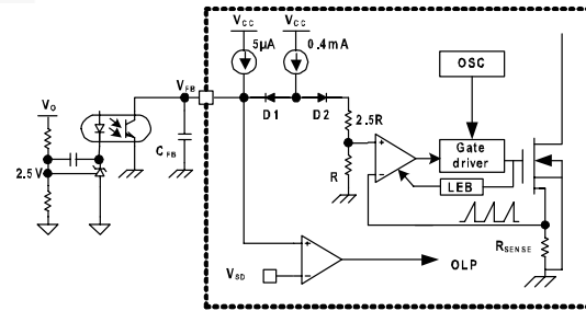
Figure 16. Pulse-Width-Modulation Circuit
