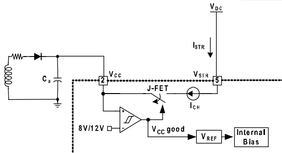
Figure 14. Startup Circuit
