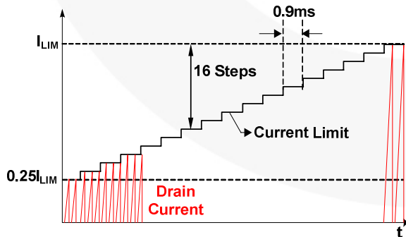
Figure 21. Internal Soft-Start
