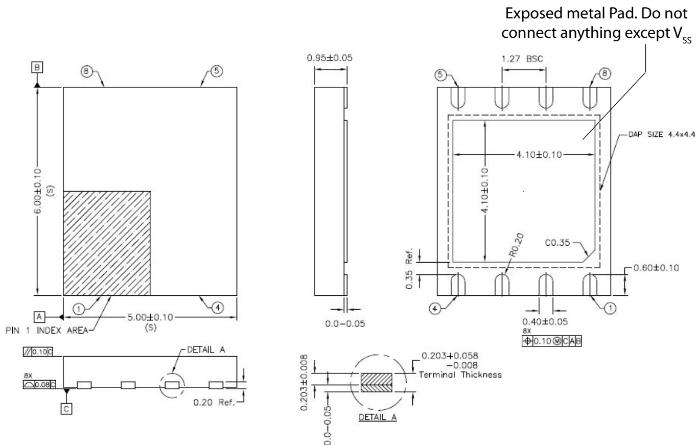
Figure 6.1 DFN Package
