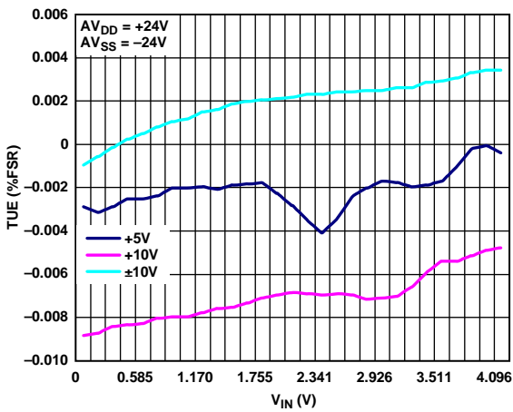
Figure 7. Total Unadjusted Error vs. V_{IN}
