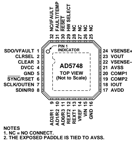
Figure 4. Pin Configuration
