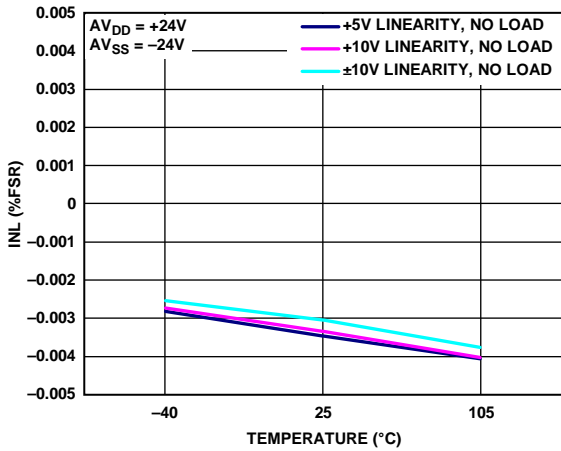
Figure 6. Integral Nonlinearity Error vs. Temperature
