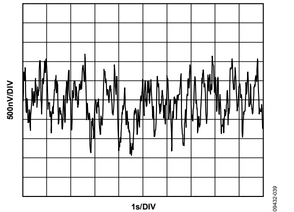
Figure 46. 0.1 Hz to 10 Hz Voltage Noise
