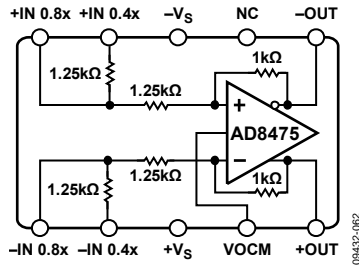
Figure 49. Block Diagram
