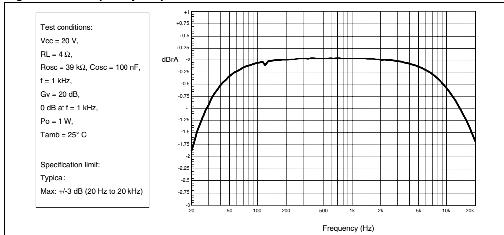
Figure 23. Frequency response
