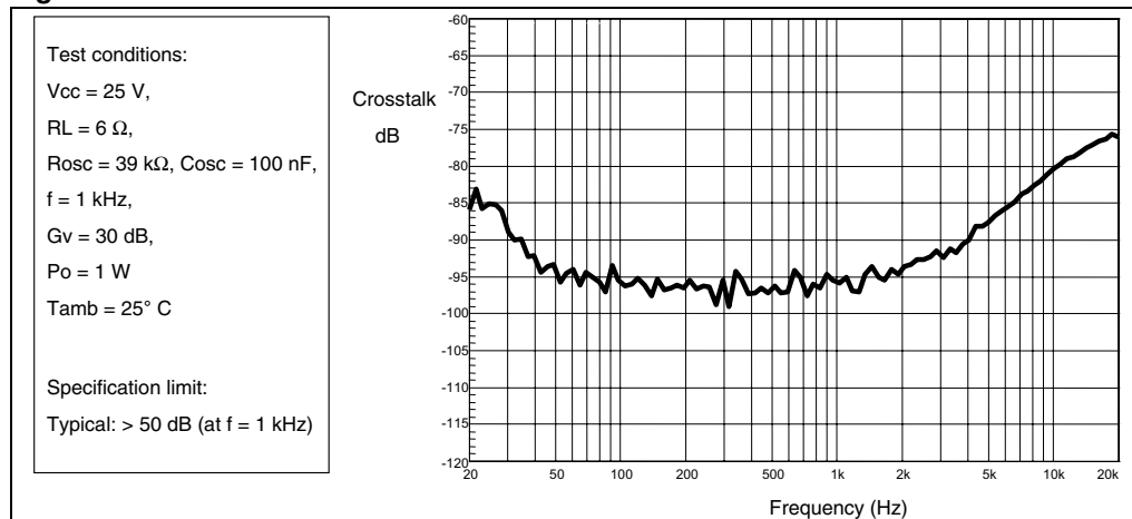
Figure 8. Crosstalk
