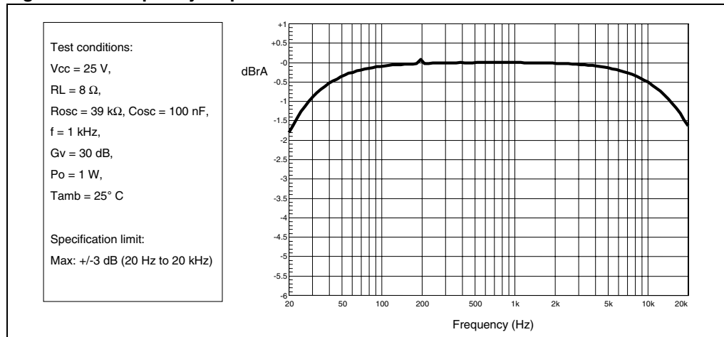
Figure 15. Frequency response
