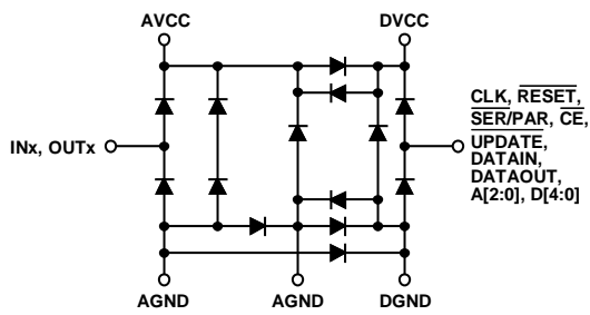
Figure 60. ESD Map
