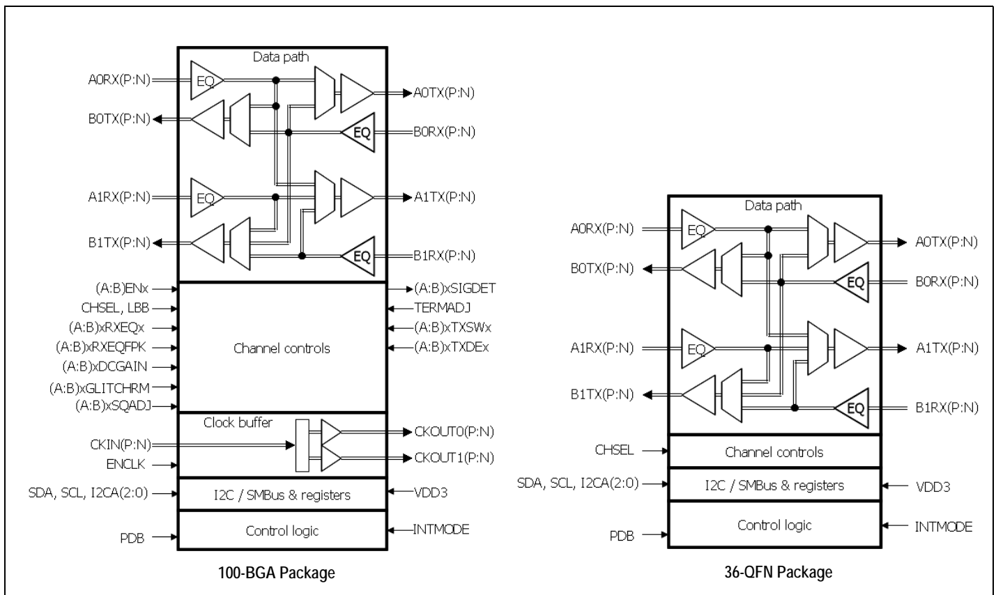
Figure 2 P0604S Block Diagrams
