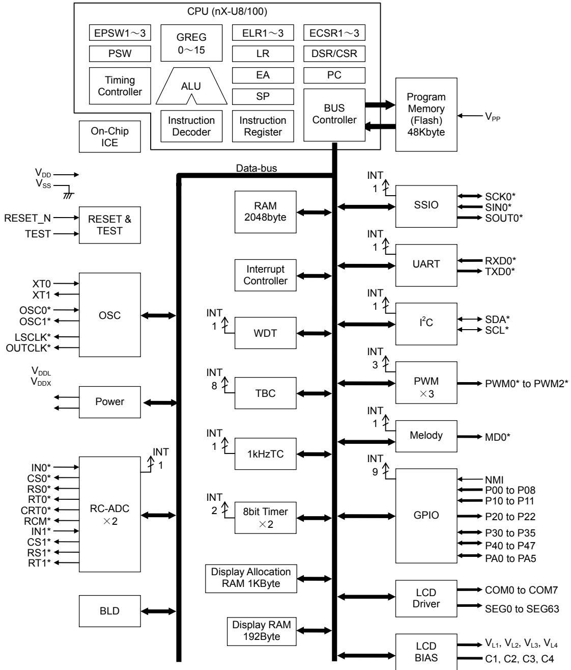
Figure 2 ML610Q429 Block Diagram
