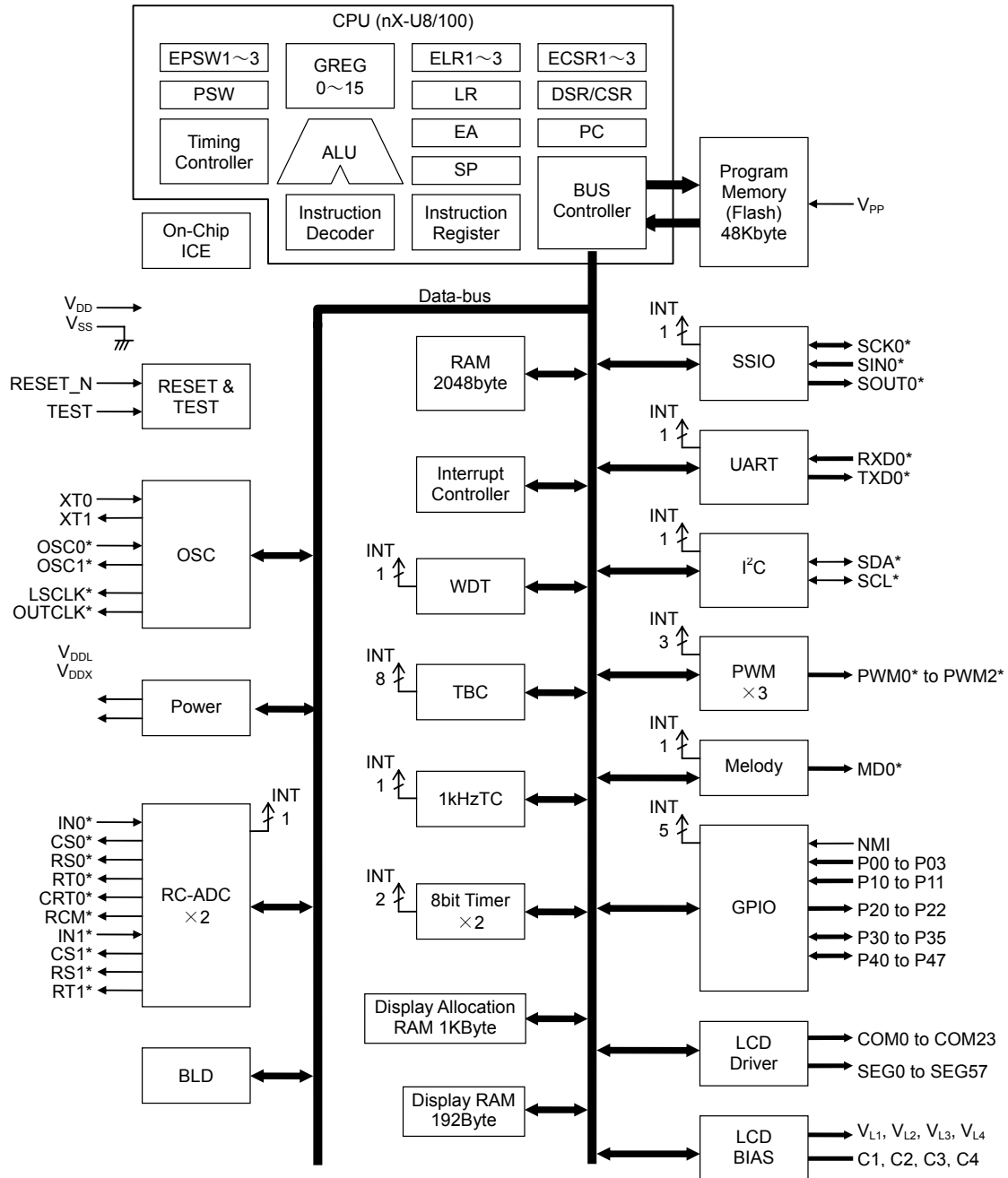
Figure 1 ML610Q428 Block Diagram
