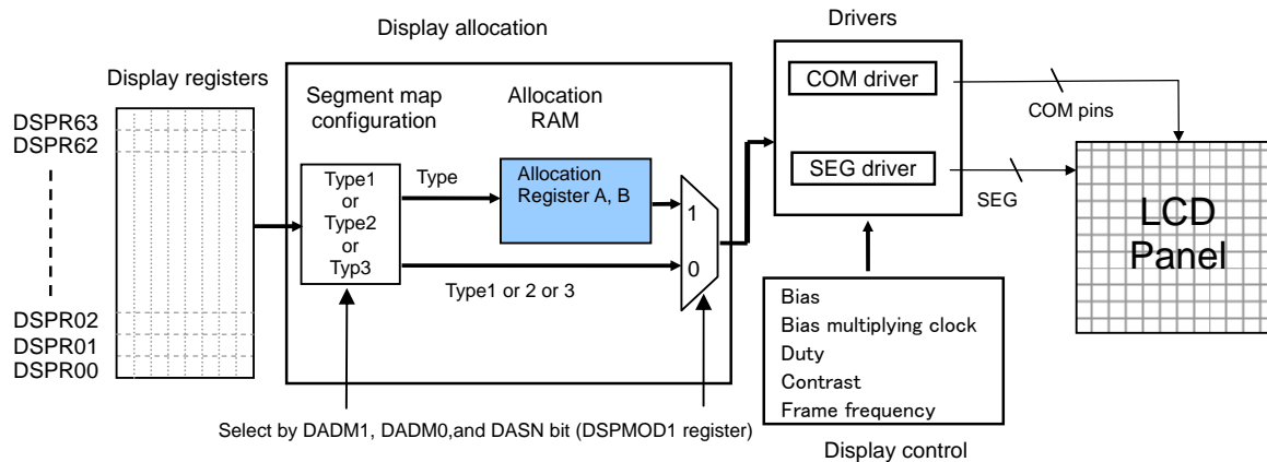
Figure 26-1 Configuration of LCD Display Function
