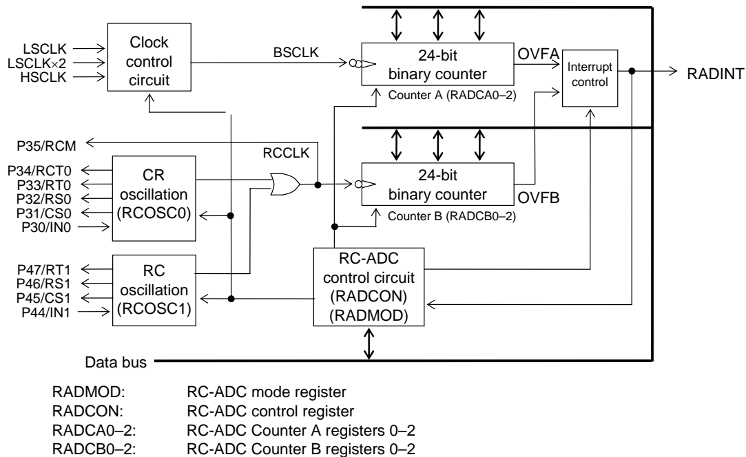
Figure 24-1 Configuration of RC-ADC
