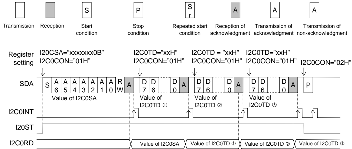
Figure 15-2 Operation Timing in Data Transmit (Write)
