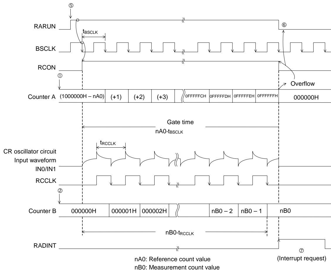
Figure 24-6 Operation Timing in Counter A Reference Mode
