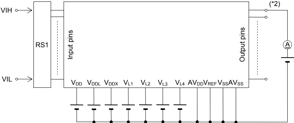
Measuring circuit 3
