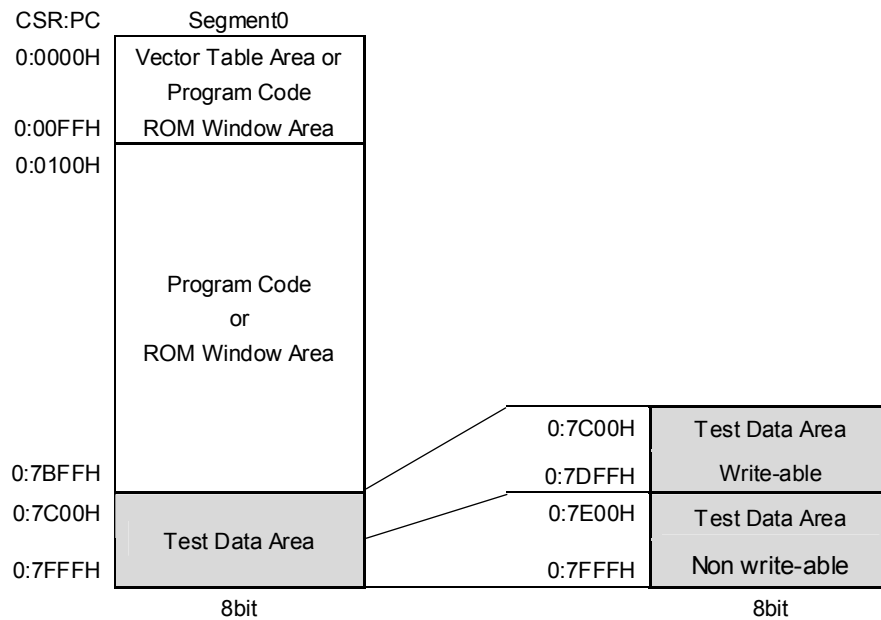
Figure 2-1 Configuration of Program Memory Space
