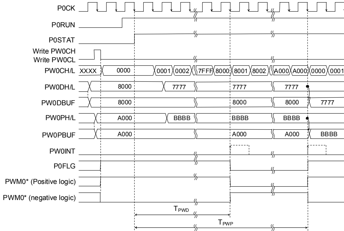
Figure 11-2 (1/2) Operation Timing Diagram of PWM0
