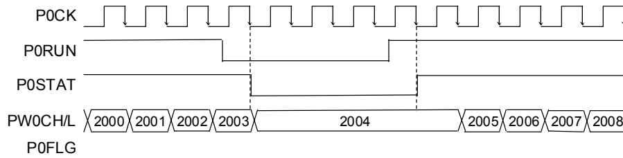
Figure 11-2 (2/2) Operation Timing Diagram of PWM0
