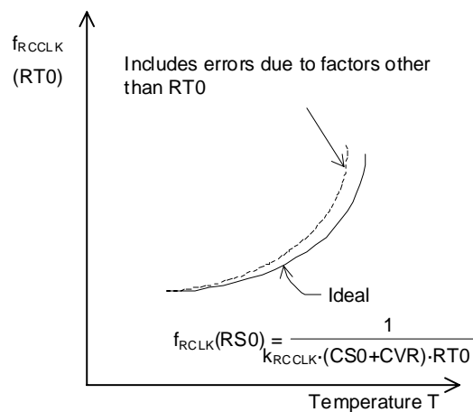
Figure 24-12 Oscillation Characteristics of Thermistor
