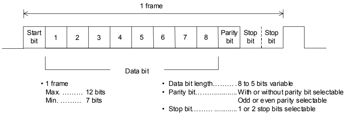
Figure 14-3 Negative Logic Input/Output Format
