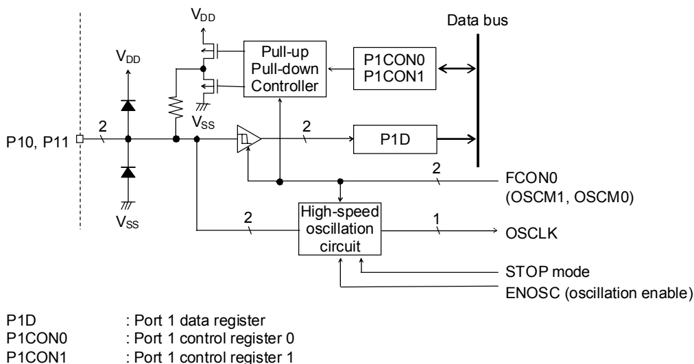
Figure 18-1 Configuration of Port 1
