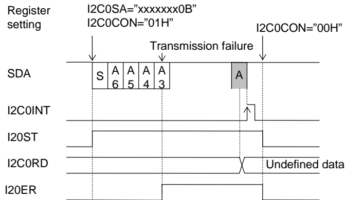
Figure 15-6 Operation Timing When Transmission Fails
