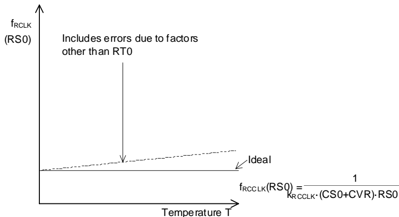
Figure 24-13 Oscillation Characteristics of Reference Resistor
