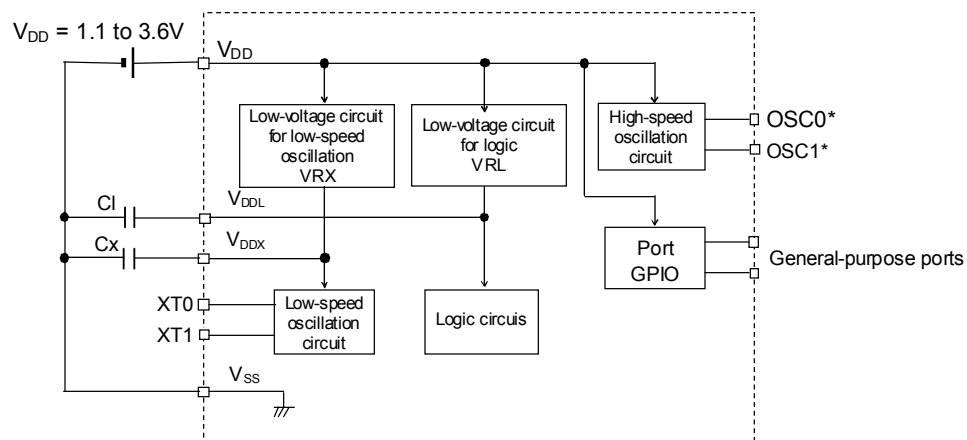
Figure 28-1 Configuration of Power Supply Circuit
