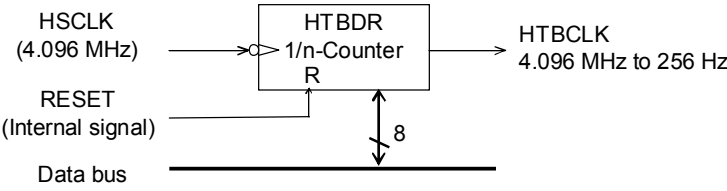
Figure 7-2 Configuration of High-Speed Time Base Counter
