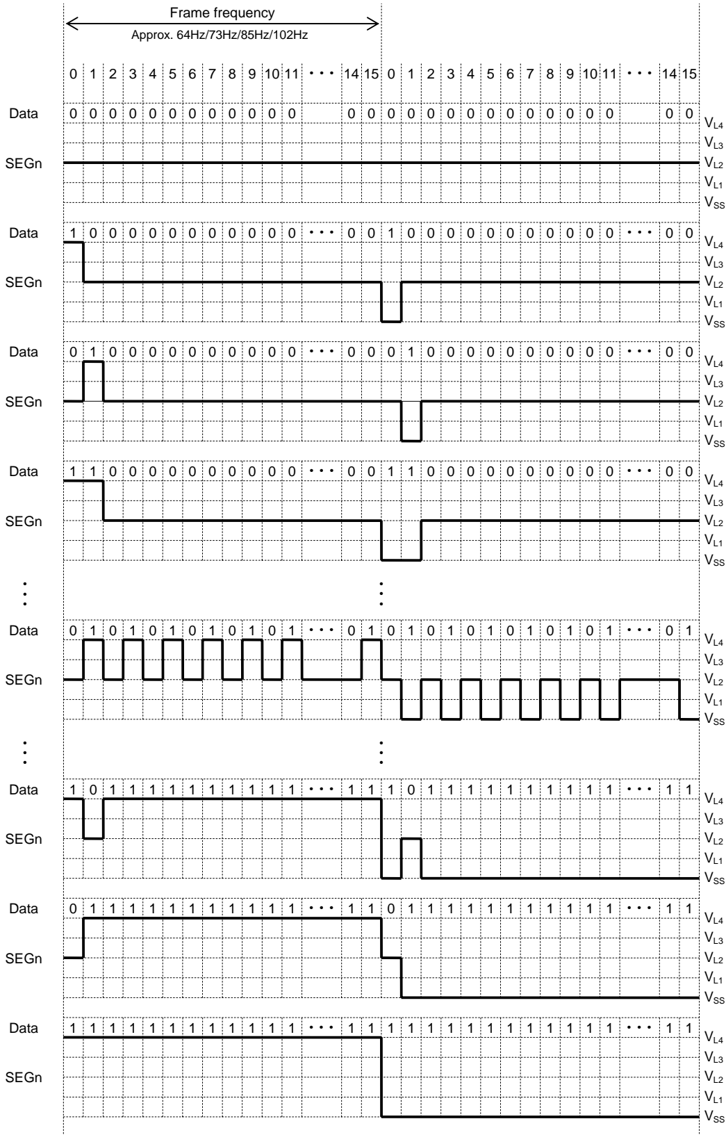
Figure 26-10 (2) Segment Output Waveforms for 1/16 Duty and 1/4 Bias
