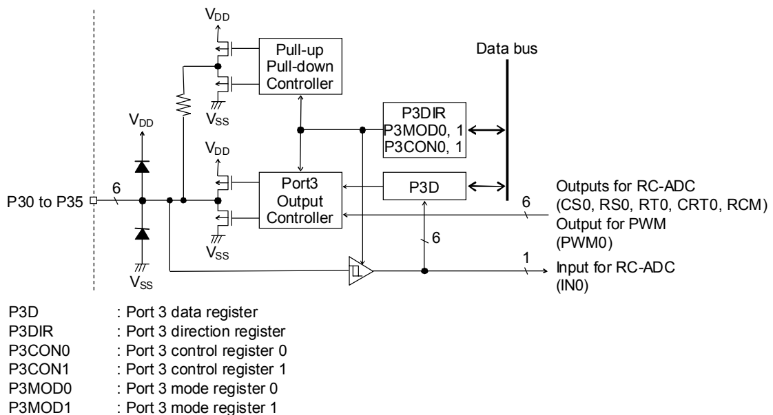
Figure 20-1 Configuration of Port 3
