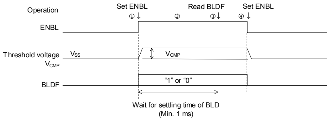
Figure 27-2 Example of Operation Timing Diagram
