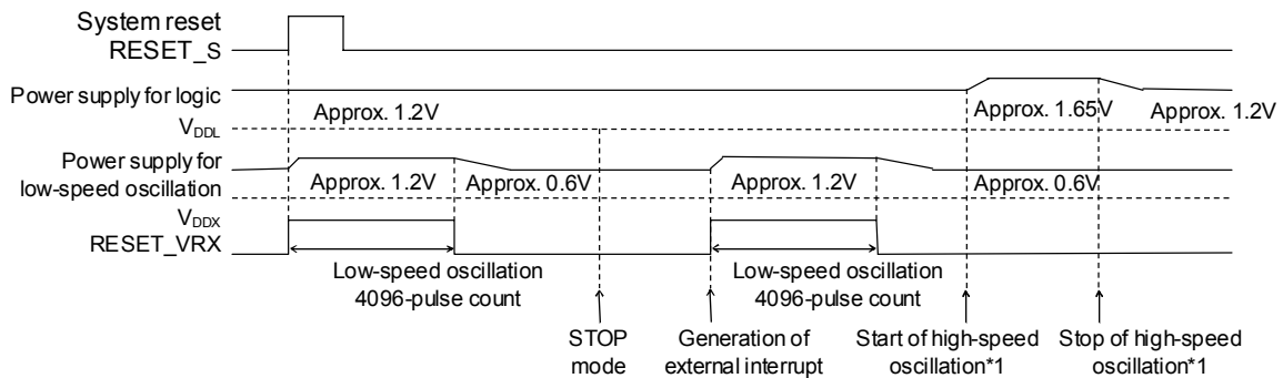
Figure 28-2 Operation Waveforms of Power Supply Circuit
