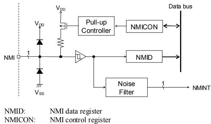
Figure 16-1 Configuration of NMI Pin
