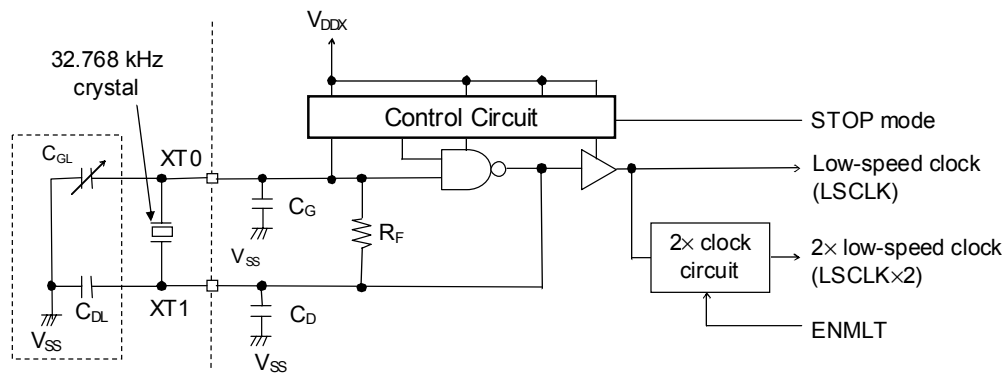
Figure 6-2 Circuit Configuration of 32.768 kHz Crystal Oscillation Mode
