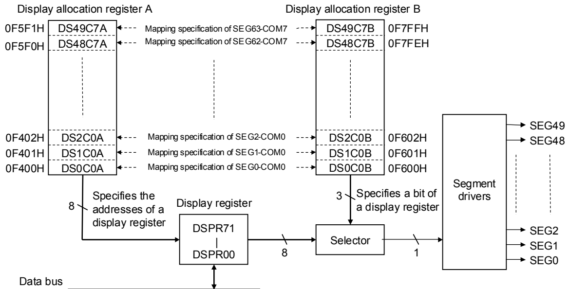
Figure 26-8 Configuration When Using the Programmable Display Allocation Function
