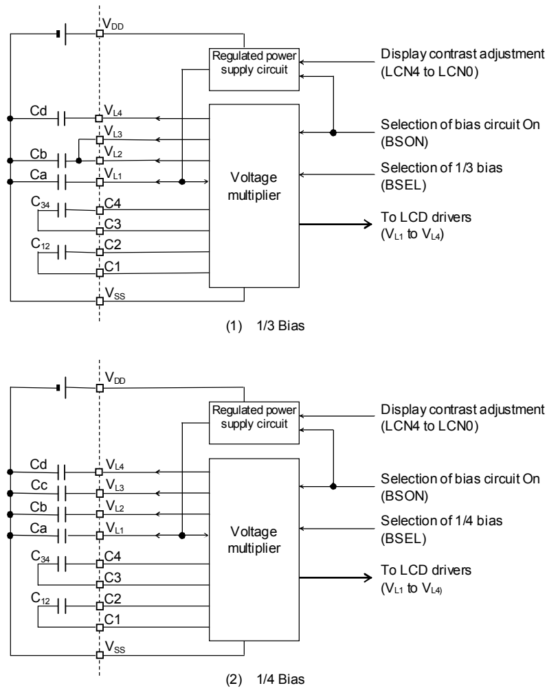
Figure 26-5 Configuration of Bias Generation Circuit
