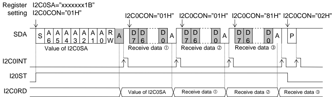
Figure 15-3 Operation Timing in Data Receive (Read)
