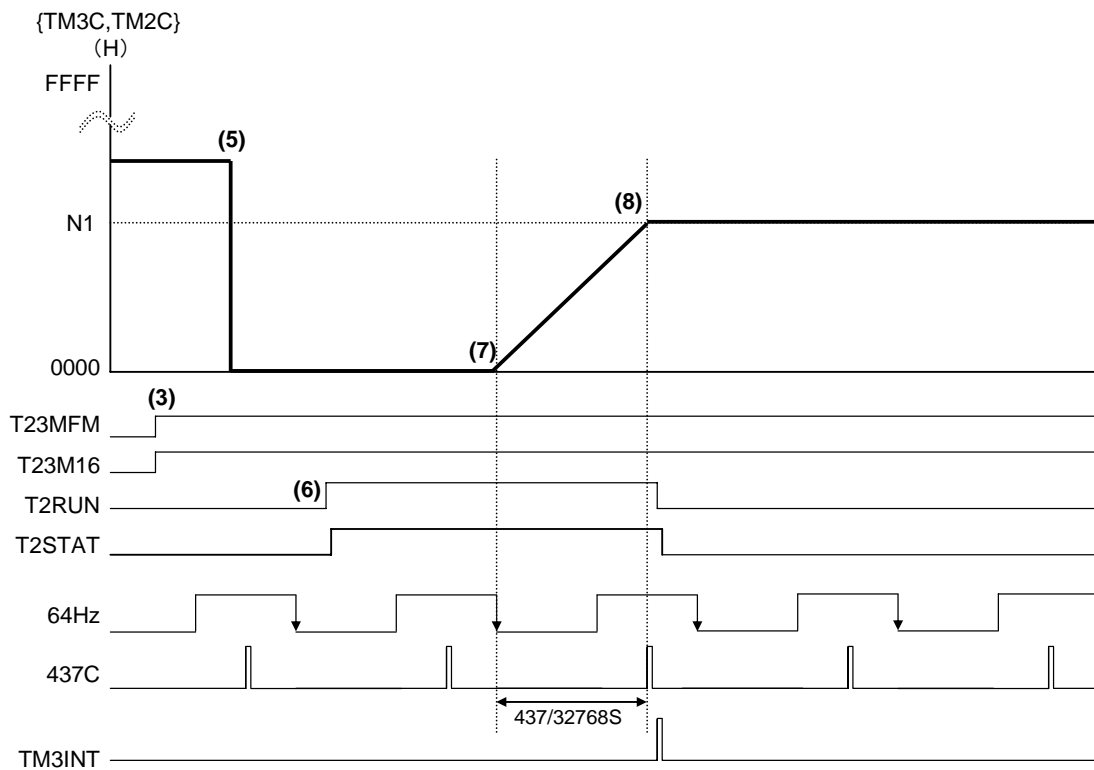
Figure 10-3 Operation Timing in frequency measurement mode
