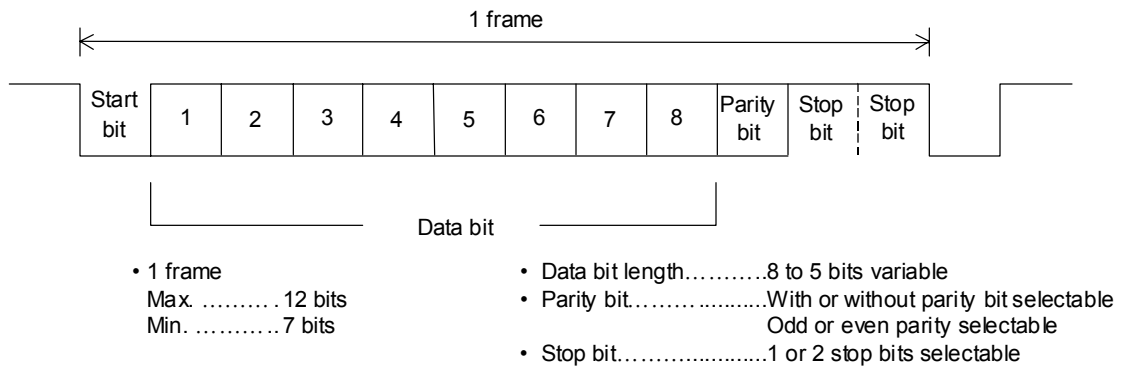
Figure 14-2 Positive Logic Input/Output Format
