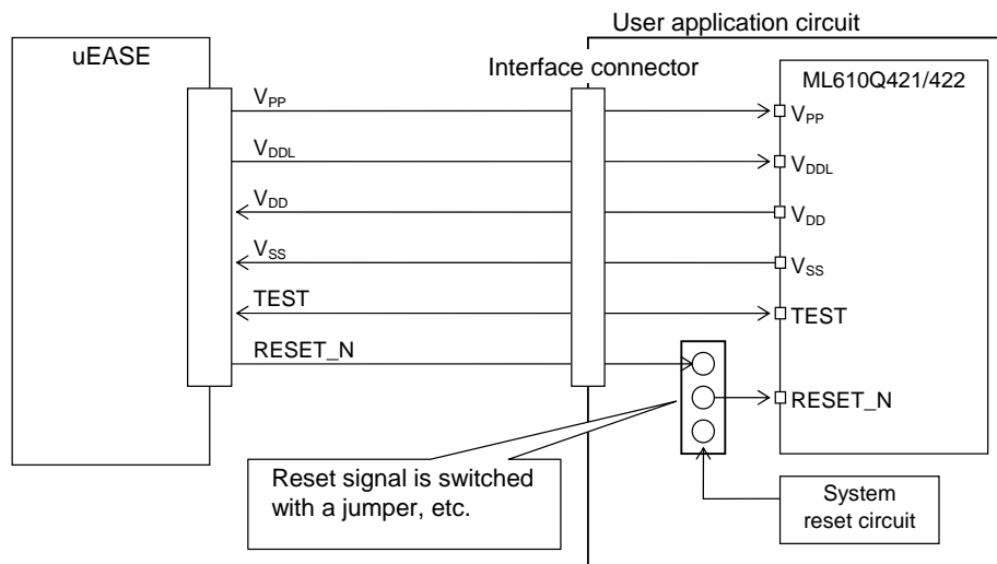
Figure 29-1 Connection to On-chip Debug Emulator (uEASE)
