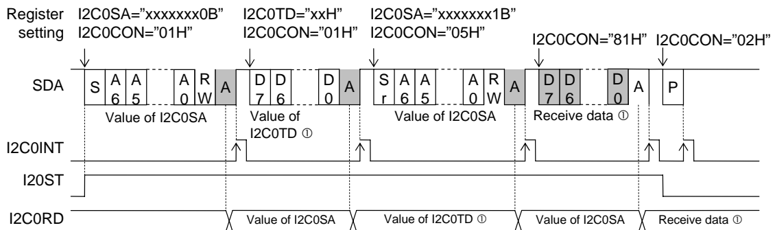
Figure 15-4 Operation Timing at Data Transmit/Receive (Write/Read) Switching
