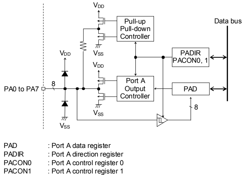
Figure 22-1 Configuration of Port A
