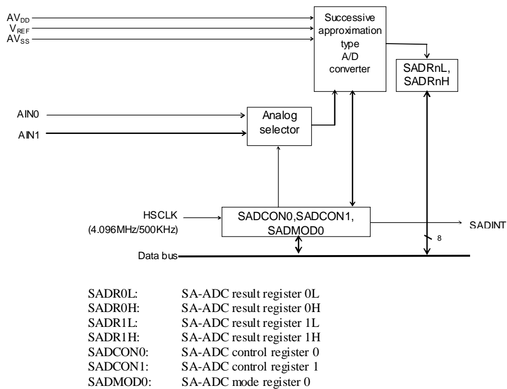
Figure 25-1 Configuration of SA-ADC
