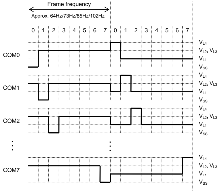
Figure 26-9 (1) Common Output Waveforms for 1/8 Duty and 1/3 Bias
