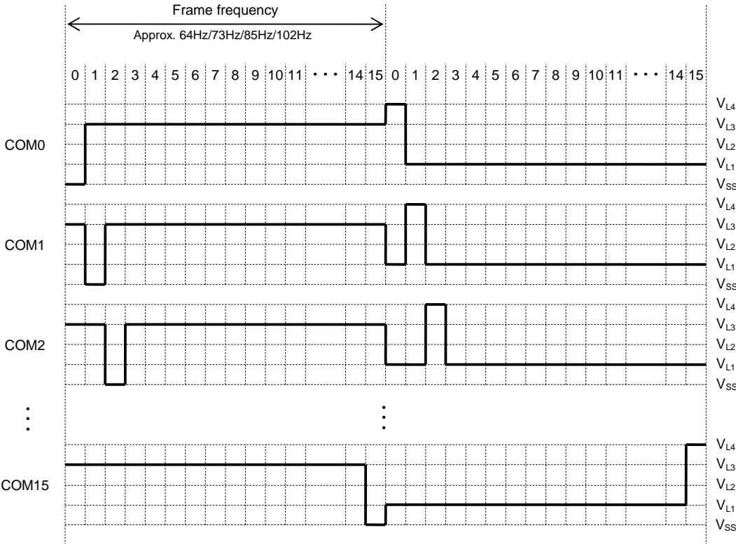
Figure 26-9 (2) Common Output Waveforms for 1/16 Duty and 1/4 Bias
