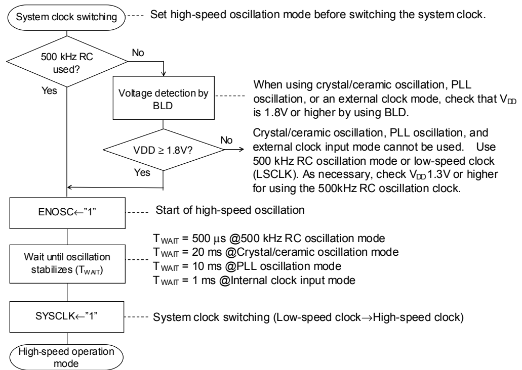
Figure 6-11 Flow of System Clock Switching Processing (LSCLK→HSCLK)
