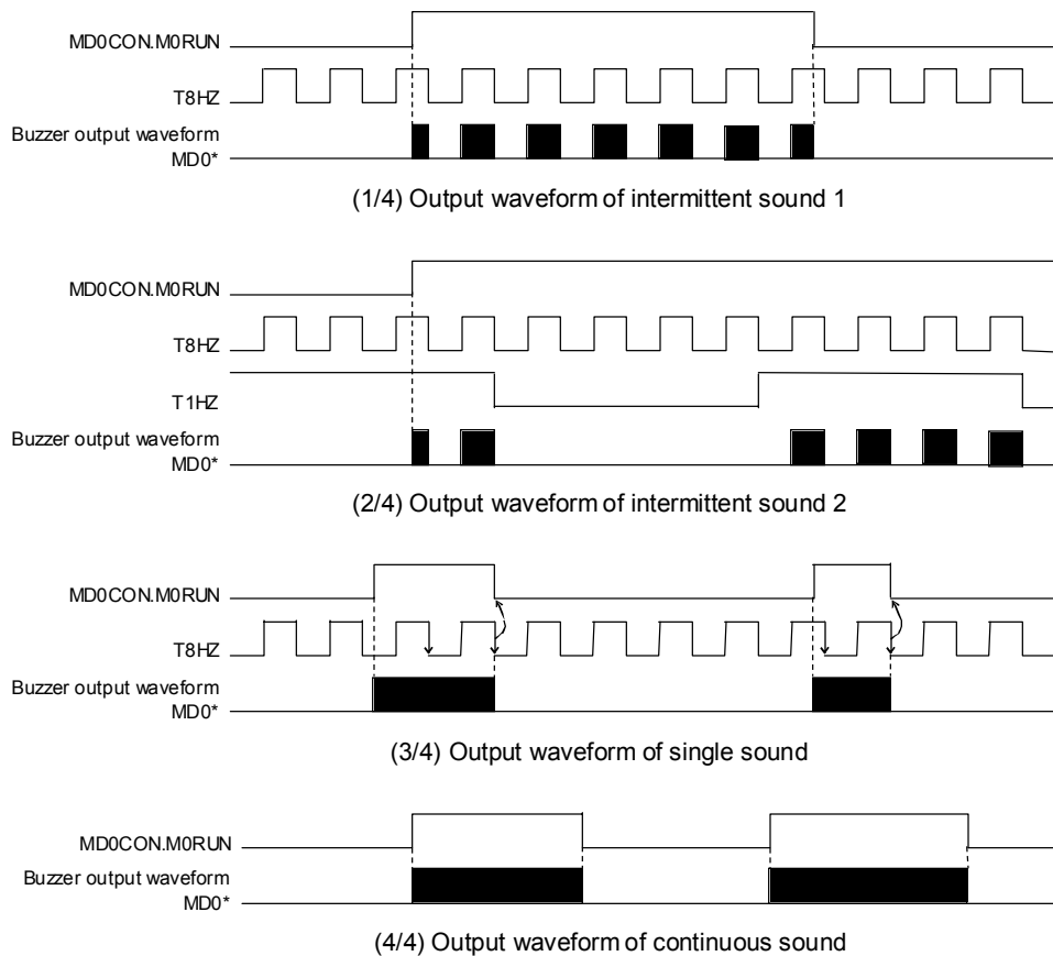
Figure 23-4 Output Waveform of Each Buzzer Output Mode
