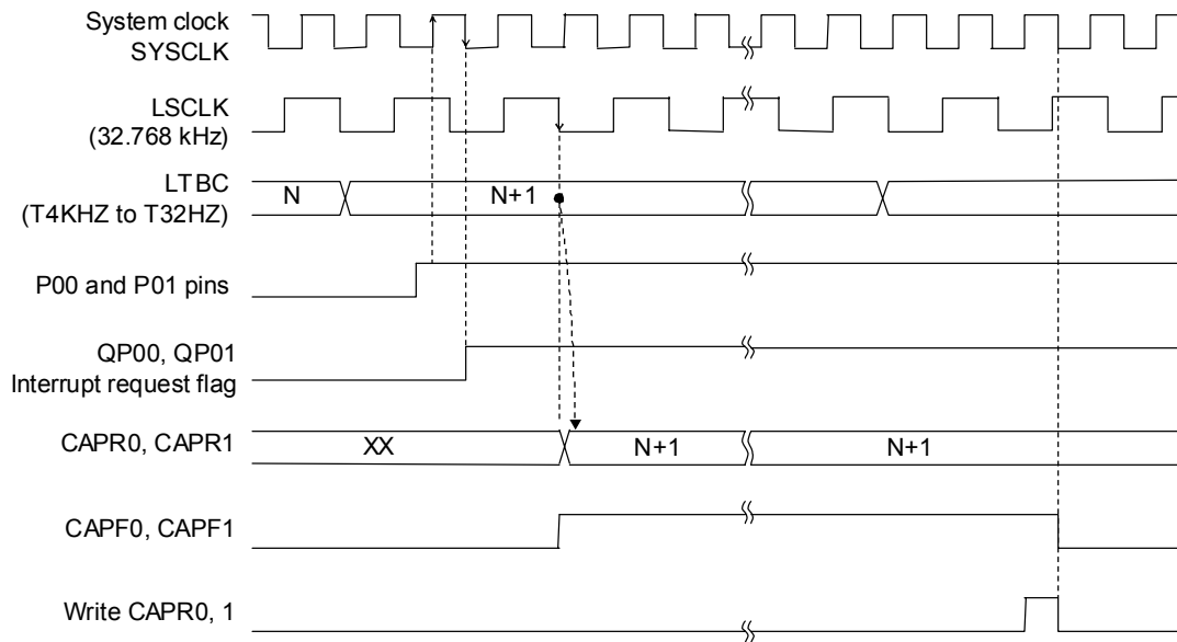
Figure 8-2 Timing Diagram of Capture Operation
