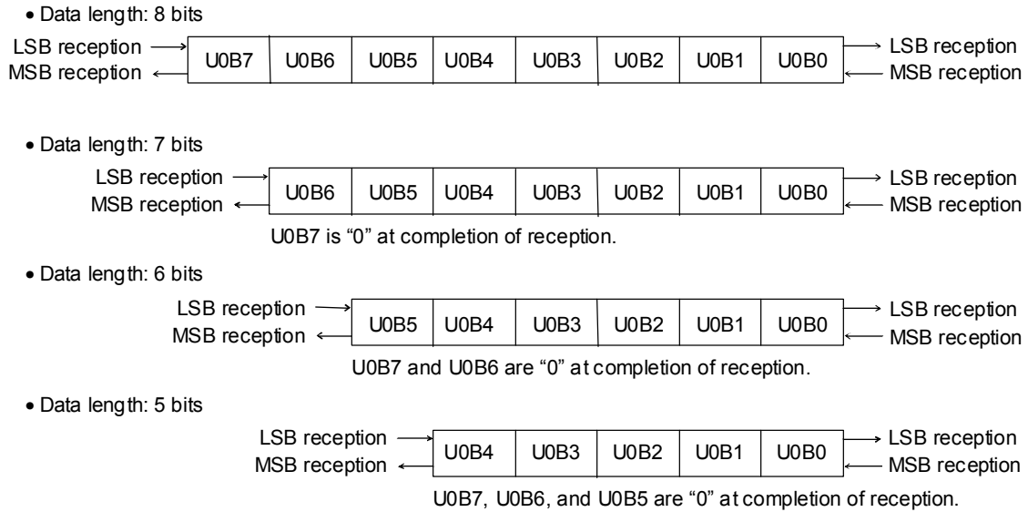
Figure 14-4 Relationship between Transmit/Receive Buffer and Transmit/Receive Data
