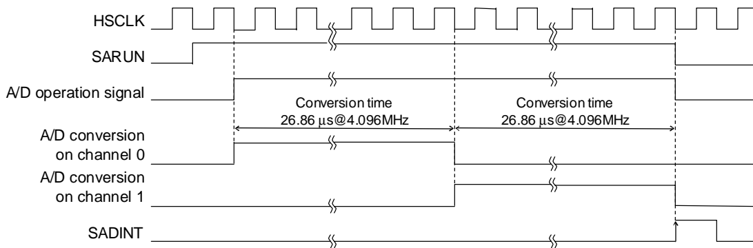
Figure 25-3 SA-ADC Operation Timing at Direct Input
