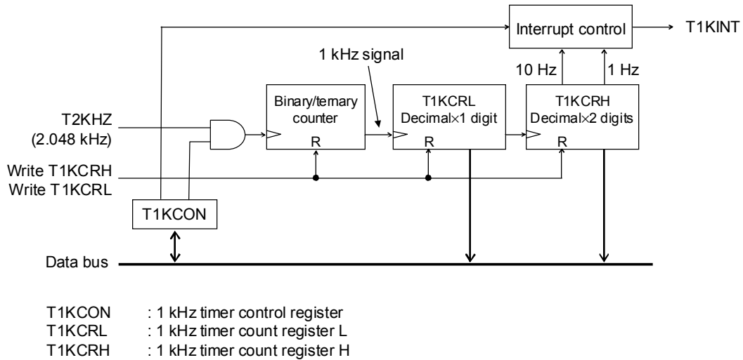
Figure 9-1 Configuration of 1 kHz Timer
