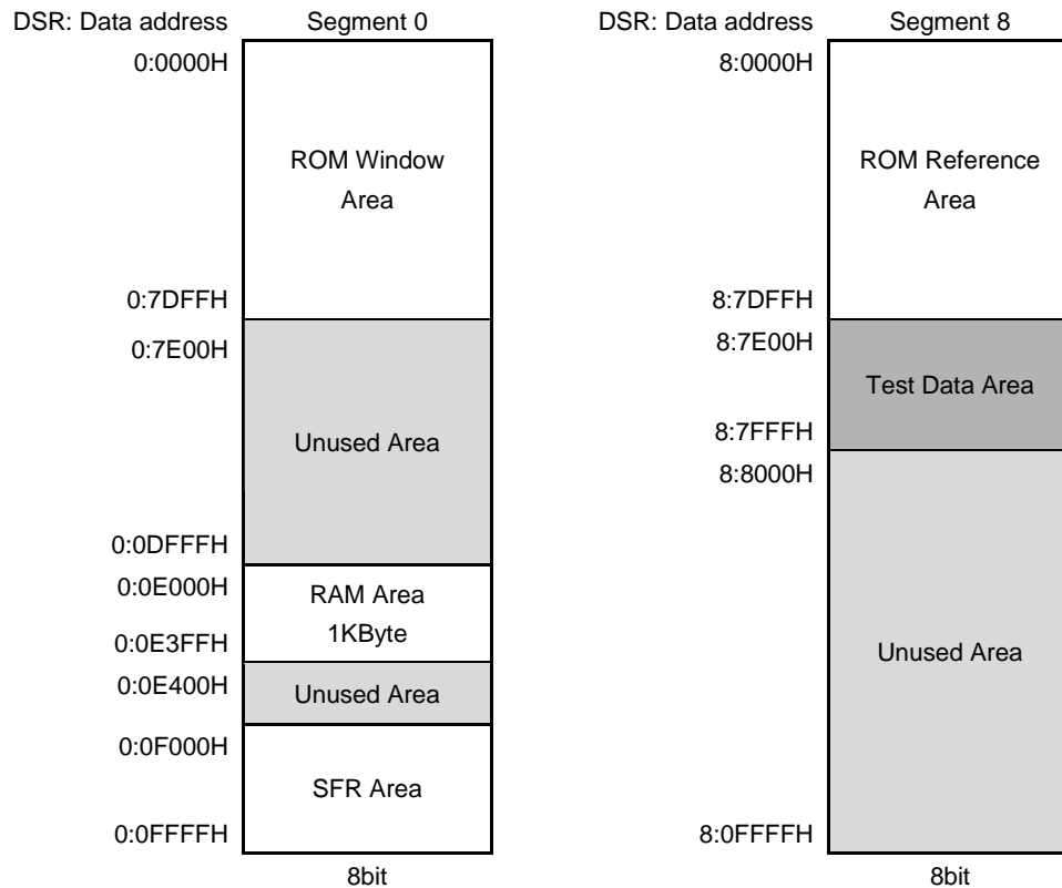
Figure 2-2 Configuration of Data Memory Space
