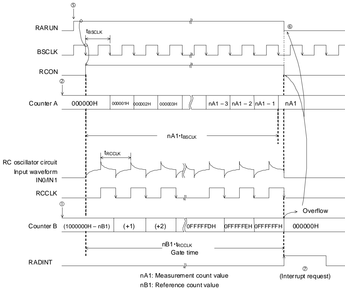
Figure 24-7 Operation Timing in Counter B Reference Mode
