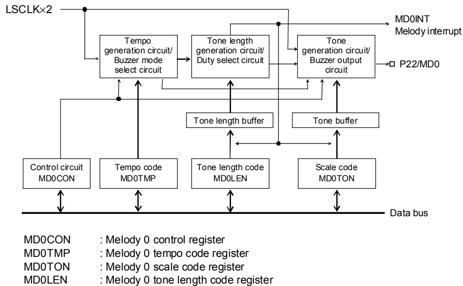
Figure 23-1 Configuration of Melody Driver
