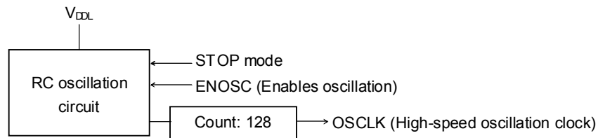
Figure 6-4 Circuit Configuration in RC Oscillation Mode
