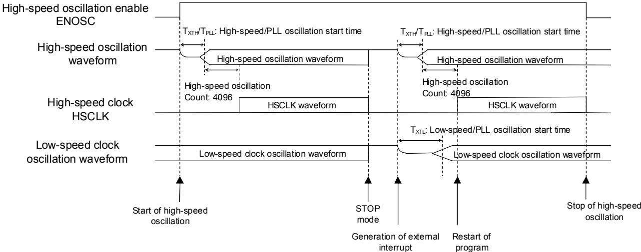
Figure 6-9 Operation of High-Speed Clock Generation Circuit in Crystal/Ceramic Oscillation Mode
