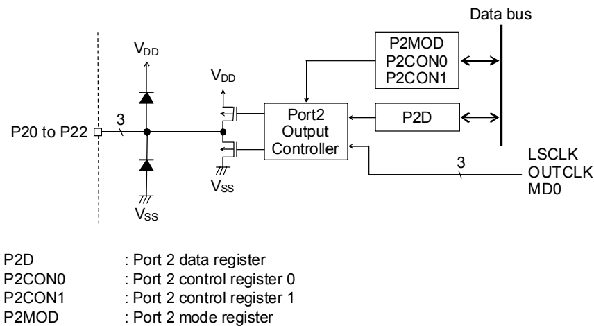
Figure 19-1 Configuration of Port 2
