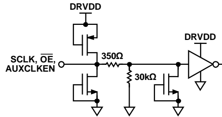
Figure 21. SCLK, OE, AUXCLKEN
