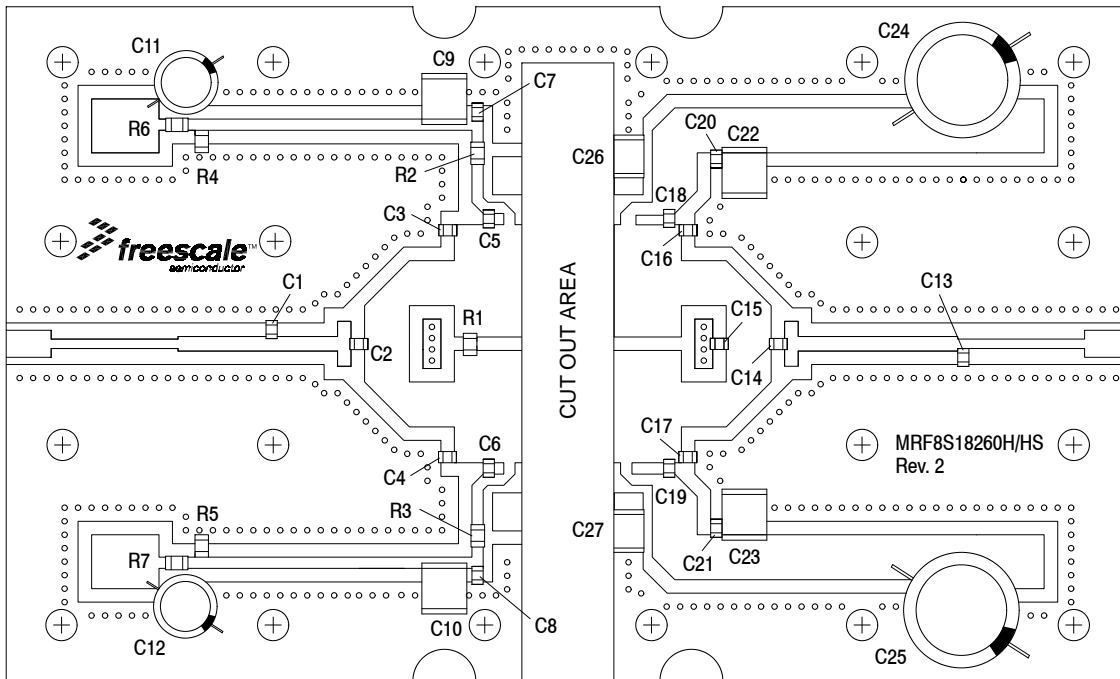
Figure 2. MRF8S18260HR6(HSR6) Test Circuit Component Layout
