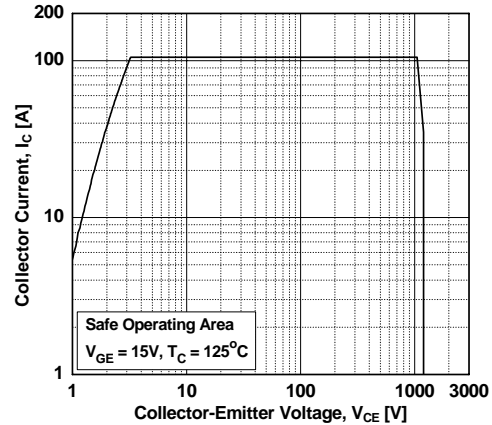
Figure 18. Turn off Switing SOA Characteristics
