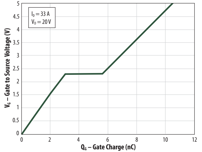
Figure 6: Gate Charge
