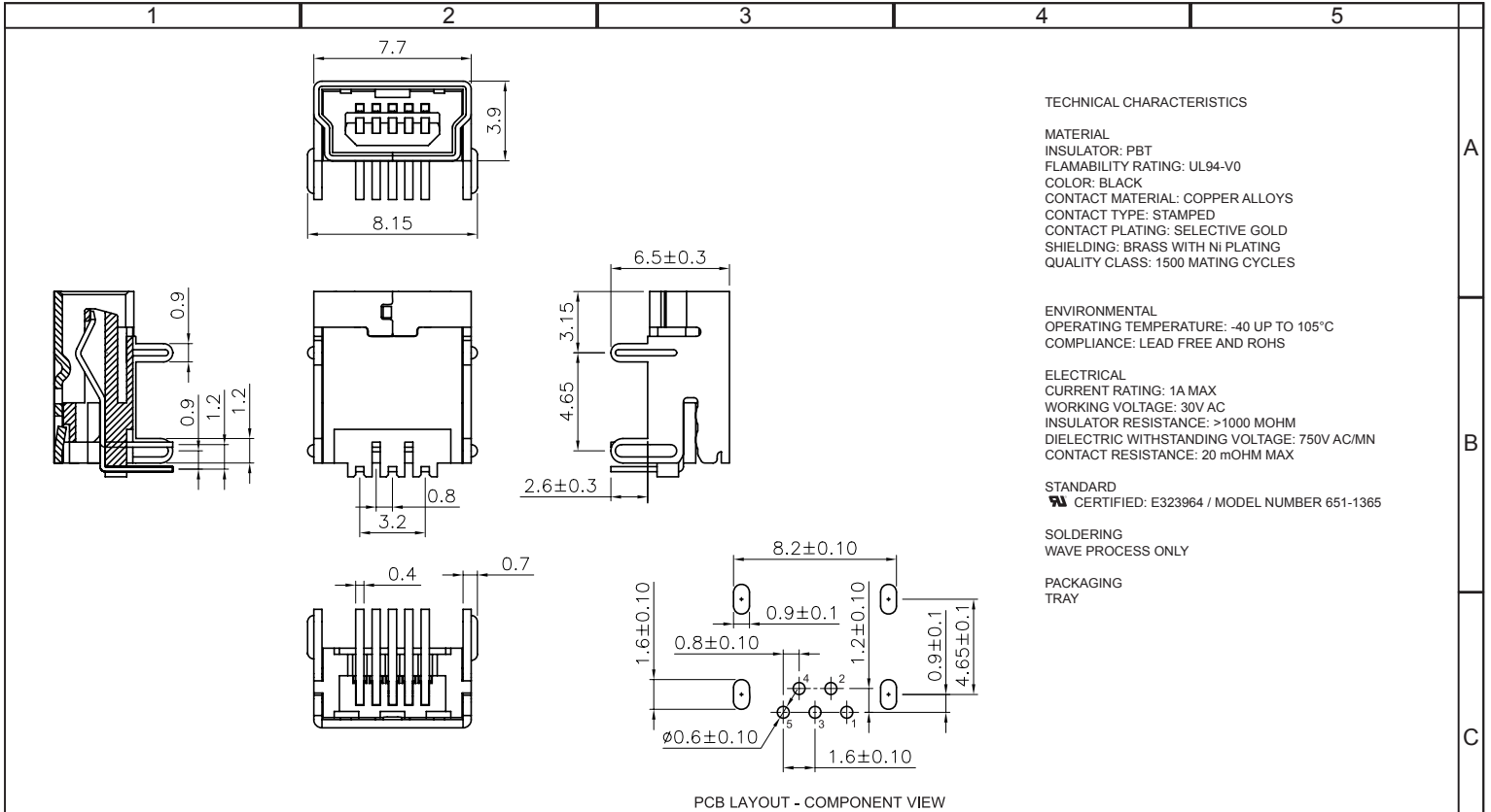
PCB LAYOUT - COMPONENT VIEW
