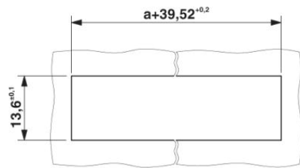
Sheet metal cutout for snap-on.
