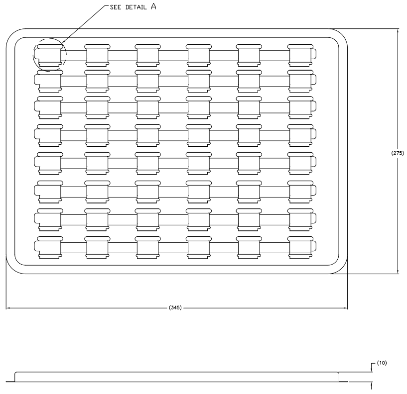
TRAY PACKAGING FOR 2041021-1 AND 2041021-3 48 PIECES PER TRAY. -NTS-
