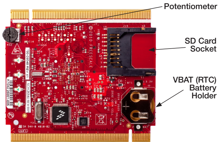
Figure 2: Back Side of TWR-K60N512 Module.
