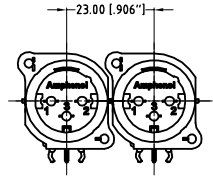
MIN MOUNTING PITCH SCALE 1:1
