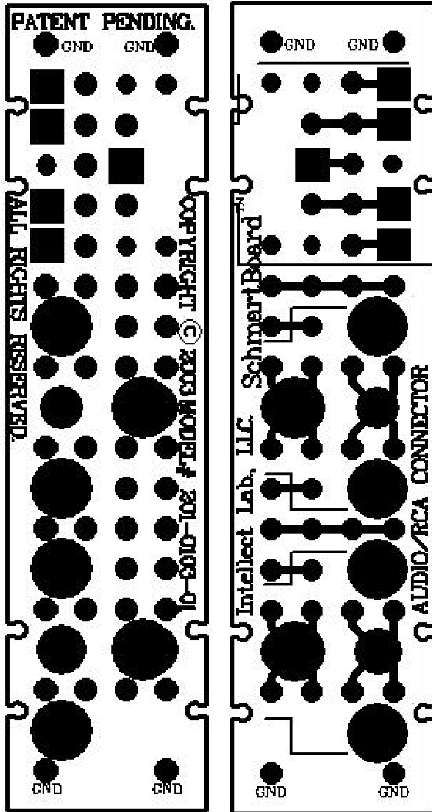
AUDIO AND RCA JACKS (201-0103-01)
