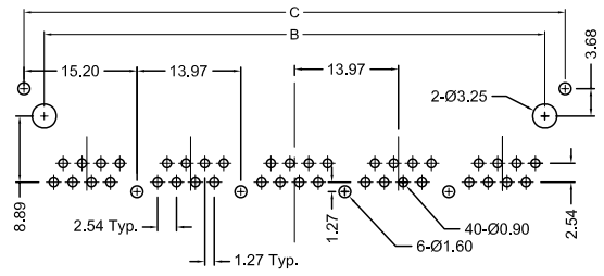
Special PCB Layout for GSGX-NS-5-88 (Top View)
