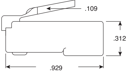
Flat Cable
