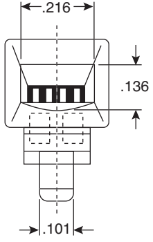
Round Cable
